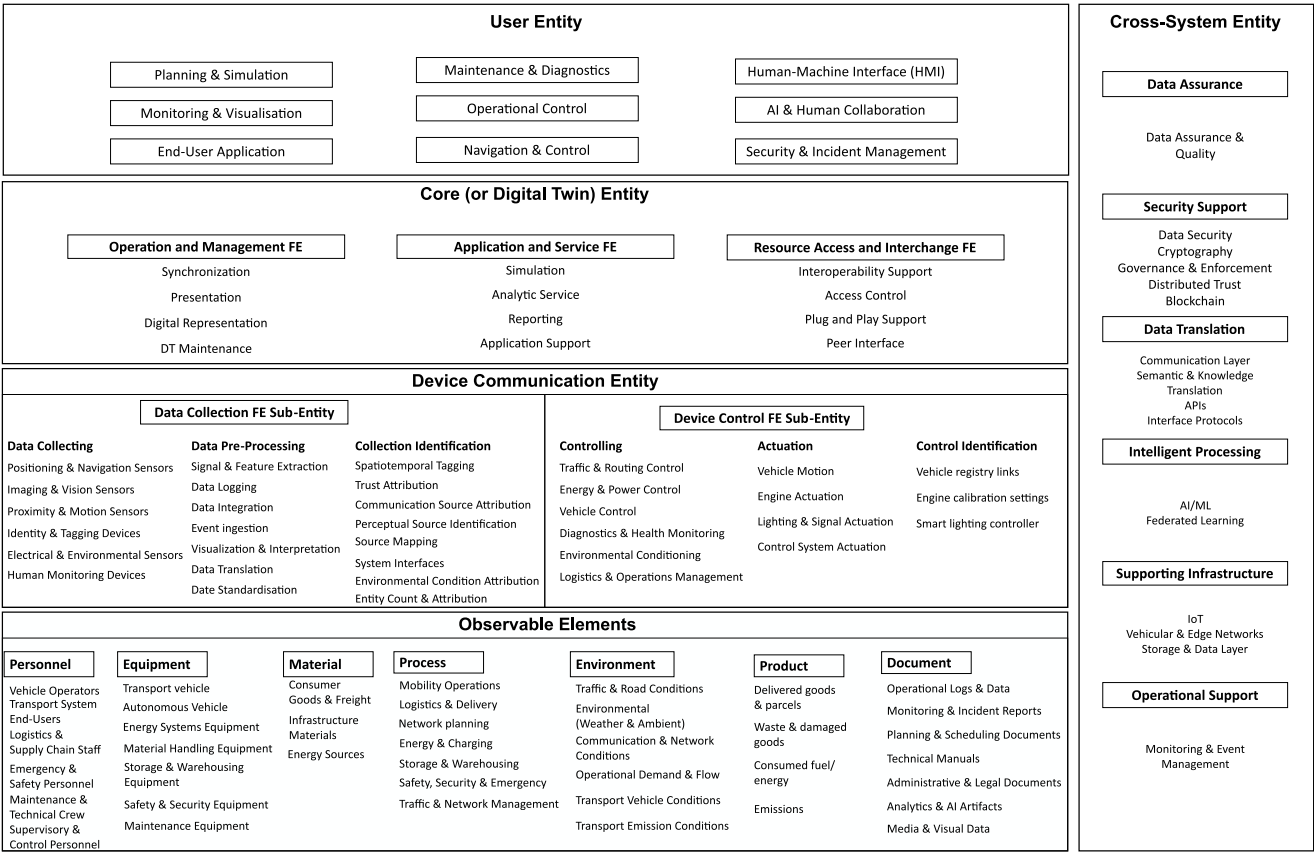
Fig. 4. Proposed ISO-23247-aligned Digital Twin framework for transport decarbonisation, presented as a reference architecture showing the main functional elements and their interaction structure.
