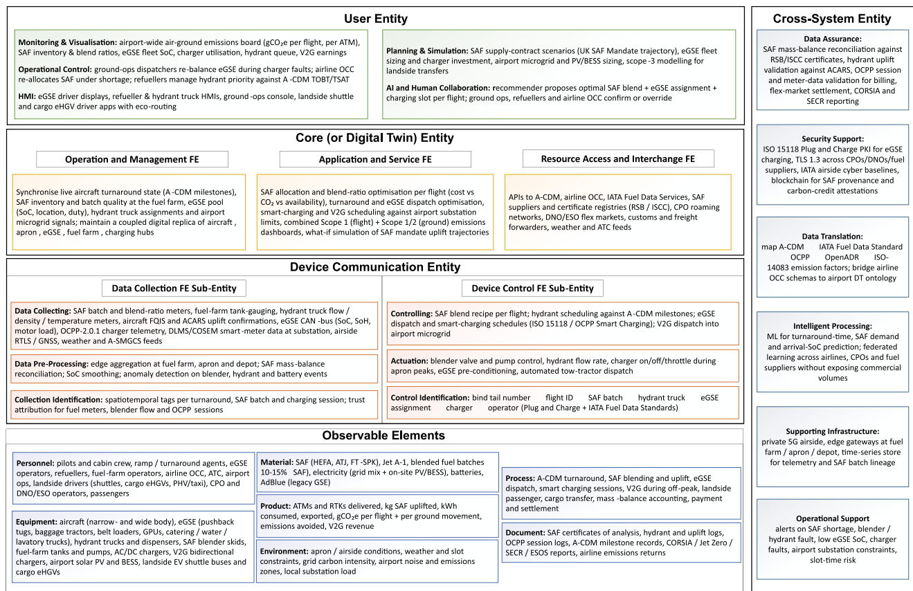
Fig. 5. ISO-23247-aligned framework as a reference architecture for a use case in Air-Road Interface for Transport Decarbonisation.
