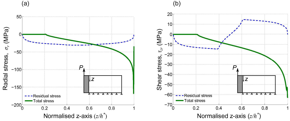
Fig. 5: Stress distribution along the pin at pin/laminate interface: dash line represents thermal residual stress after the curing process, solid line is the total stress at the peak pullout load. (a) Normal (radial) stress, \sigma_r ; (b) Shear stress, \tau_{zr} .
