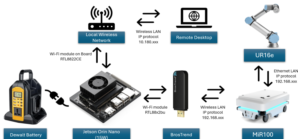
Figure 9. Hardware connection.
