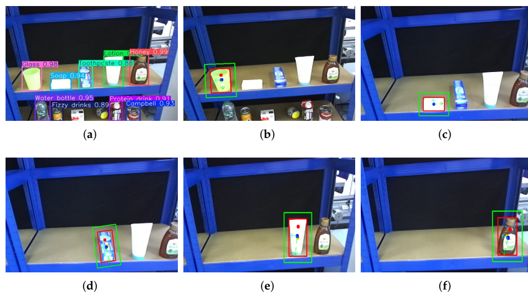
Figure 19. These are the detection and image processing results: (a) detection result from Yolov11n; (b) the object pose estimation of glass; (c) the object pose estimation of soap; (d) the object pose estimation of toothpaste; (e) the object pose estimation of lotion; (f) the object pose estimation of honey.
