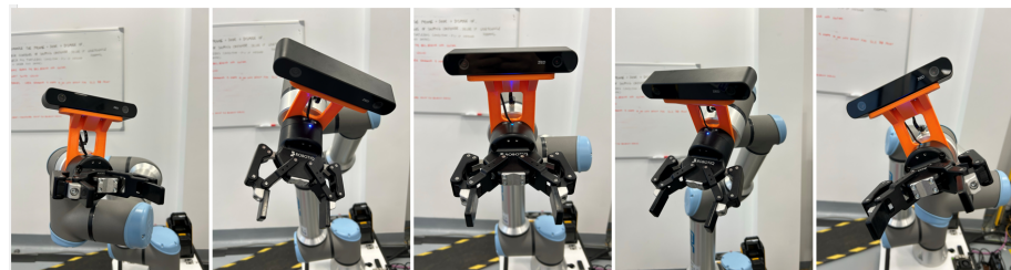
Figure 13. Robot orientation Control.
