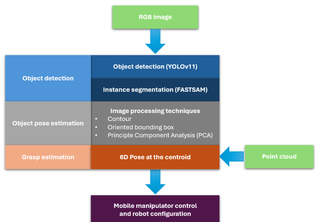
Figure 1. System architecture.
