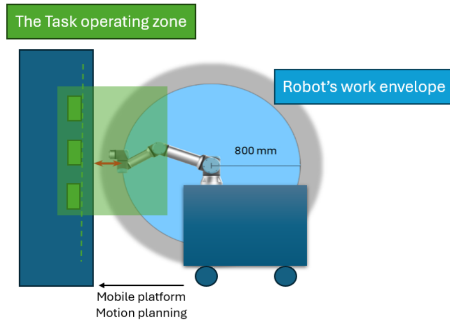
Figure 12. Work envelope.
