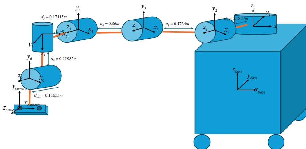
Figure 10. Initial pose (UR16e).
