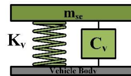
Figure 3. 1-DOF passive suspension system (PS)
