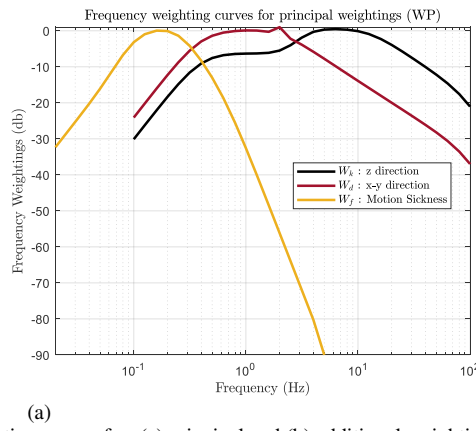
Figure 8. Frequency weighting curves for: (a) principal and (b) additional weighting
