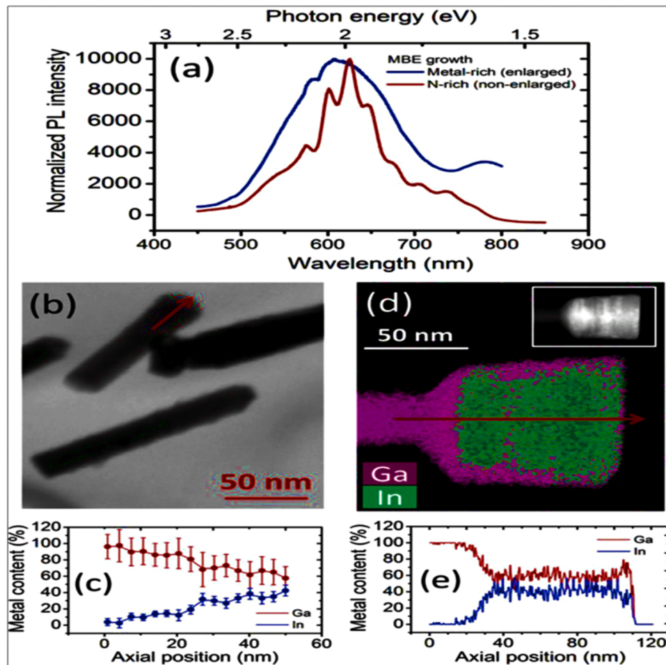
Fig. 5. (a) Macro-photoluminescence spectra of InGaN Nanowires (NWs) emitting in the 600 nm range in nitrogen-rich (non-enlarged) and metal-rich (enlarged) conditions, respectively. (b), (d-inset) Scanning electron microscopy images of InGaN NWs grown in nitrogen-rich and metal-rich conditions, respectively. (d) In and Ga Energy-Dispersive X-ray (EDX) mapping of the InGaN section grown in metal-rich conditions. (c), (e) In and Ga concentration profiles along the growth axis of InGaN NWs grown in nitrogen-rich and metal-rich conditions, respectively [53].
