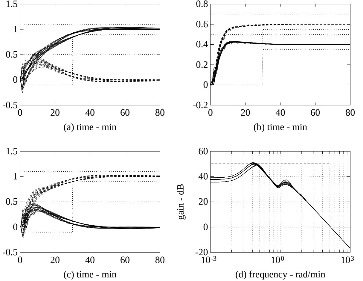
Figure 3: Responses of y_1 (—) and y_2 (- - -) of all extreme plants to (a) input h(t) \begin{bmatrix} 1 \\ 0 \end{bmatrix} , (b) input h(t) \begin{bmatrix} 0.4 \\ 0.6 \end{bmatrix} , (c) input h(t) \begin{bmatrix} 0 \\ 1 \end{bmatrix} and (d) maximum singular values of all extreme plants for (I - KG)^{-1}W_1K_p .
