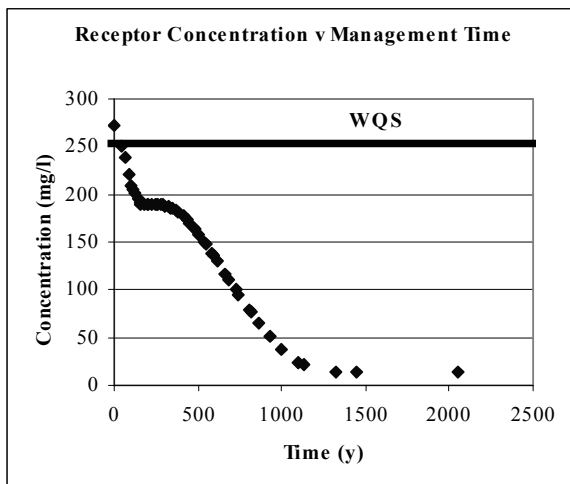
Figure 1 - Receptor concentration verses length of management time (Cd)
