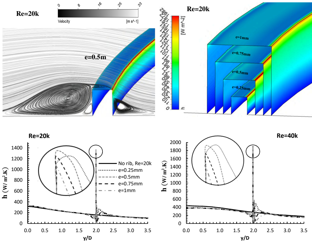
Fig. 13 Effect of rib height on local Nusselt number for Re= 20k and 40k, H/D=6
