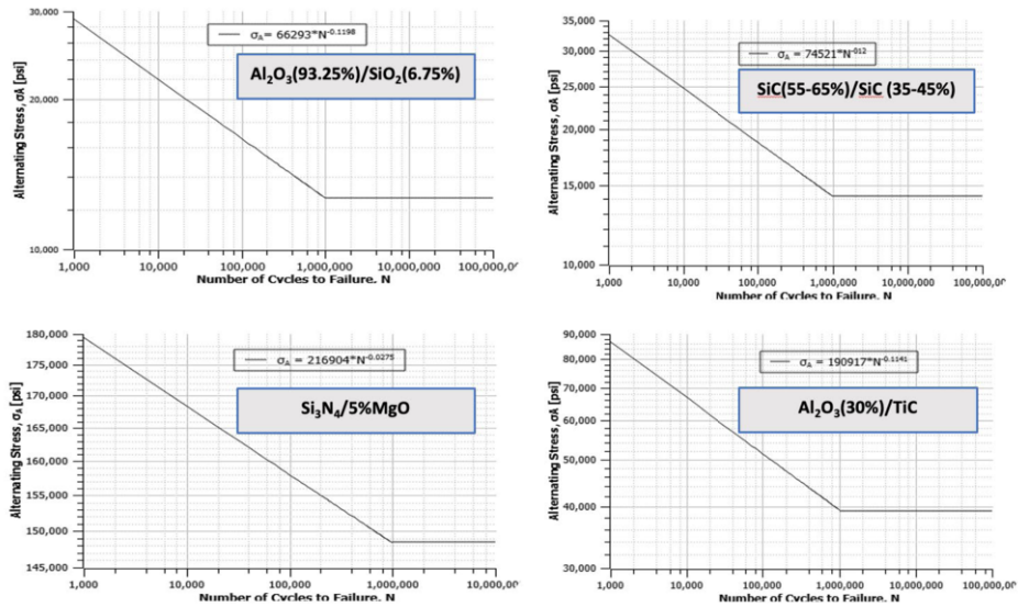
Figure 5. Alternating Stress vs Number of Cycles to failure of four different ceramic composite materials
