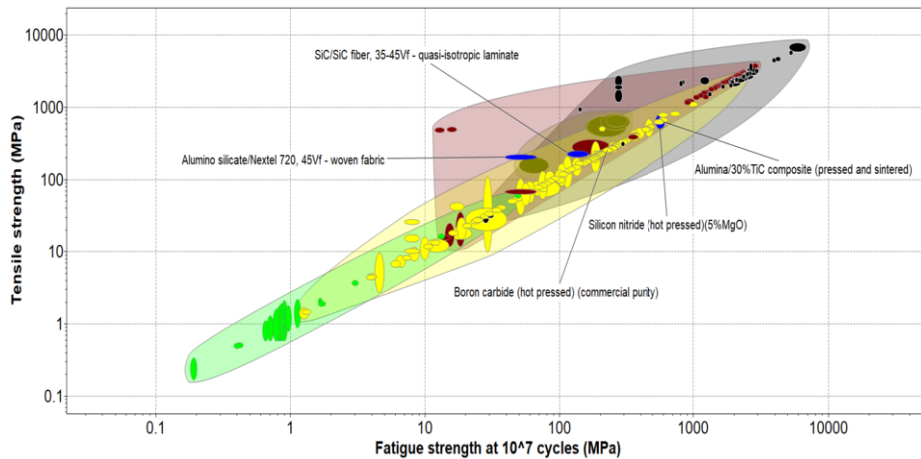
Figure 4. Tensile Strength vs Fatigue Strength comparison of Ceramics.
