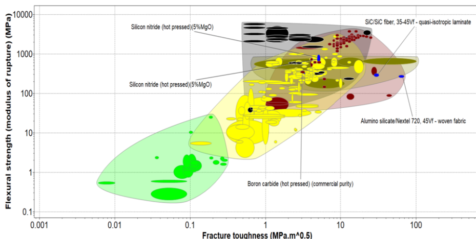
Figure 3. Flexural Strength vs Fracture Toughness comparison of Ceramics.
