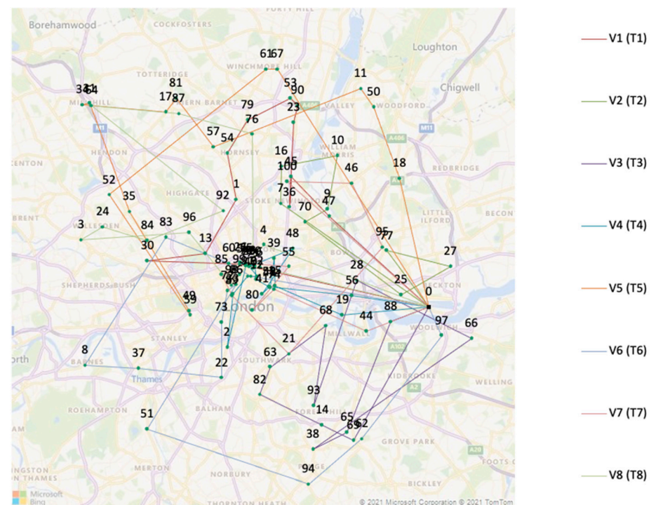
Figure 8. Visualization spreadsheet.
