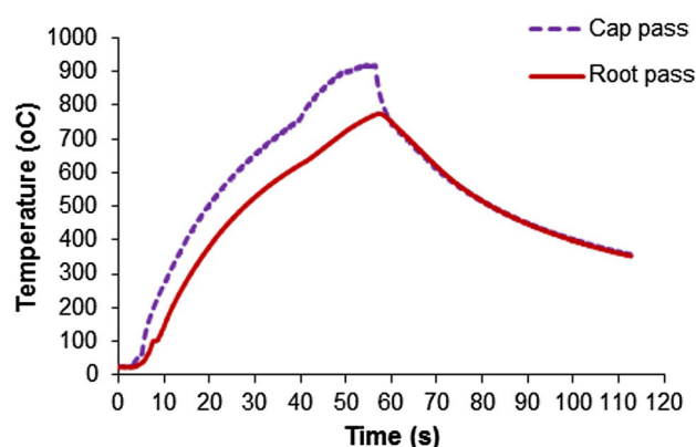
Fig. 5 Thermal cycles of control laser power using a constant beam diameter of 110 \text{ mm}
