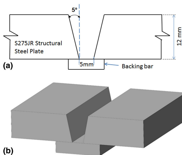
Fig. 1 S275JR structural steel plate welding set-up (a) side view (b) 3D view
