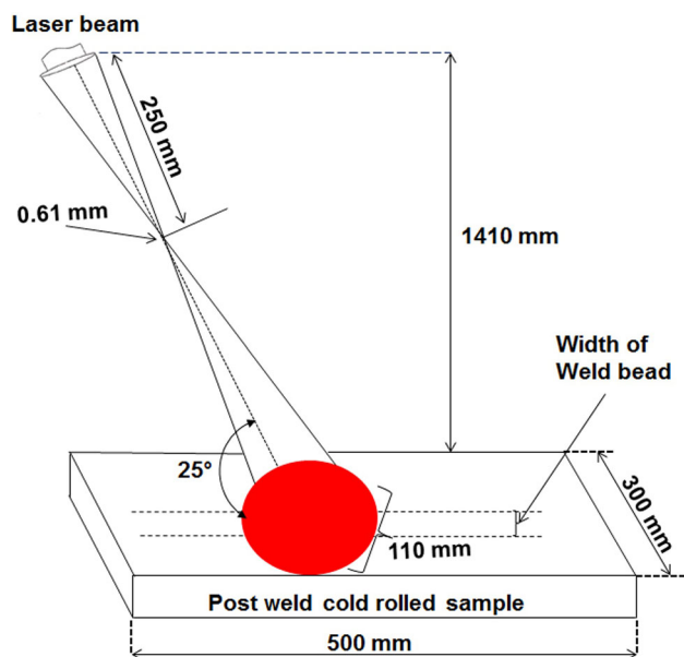
Fig. 3 Schematic diagram of laser processing set-up
