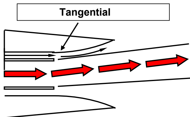
Fig 4 - Flapless Controls
