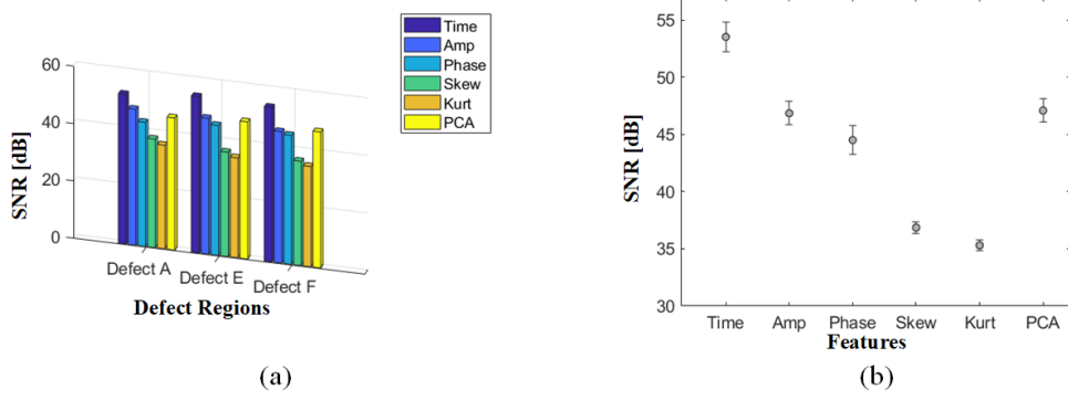
Fig.7. SNR calculated for feature selection. (a) SNR on the defective region of each feature, and (b) average SNR of each feature.
