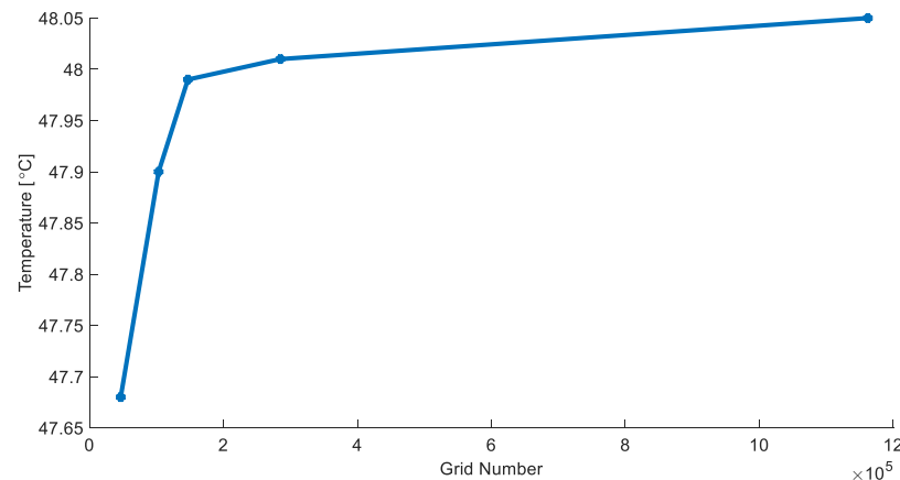
Figure 2. Mesh independence test showing variation in temperature with the grid number.
