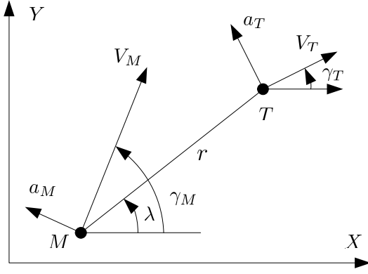
Fig. 1. Planar engagement geometry.
