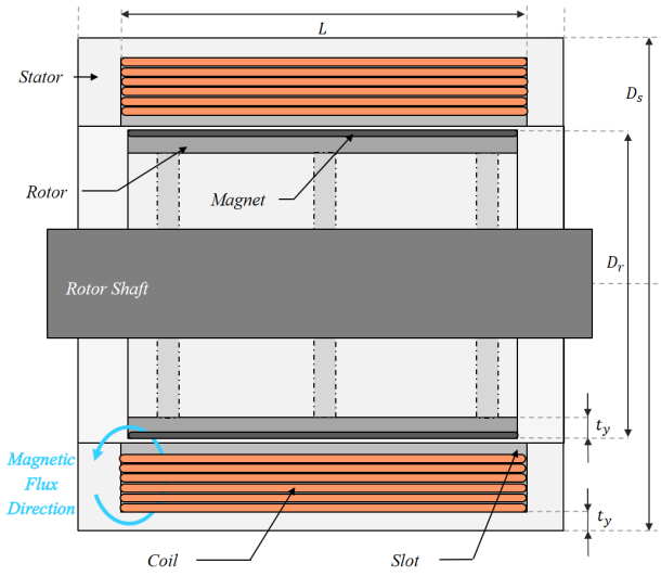
(b) Front cut view
