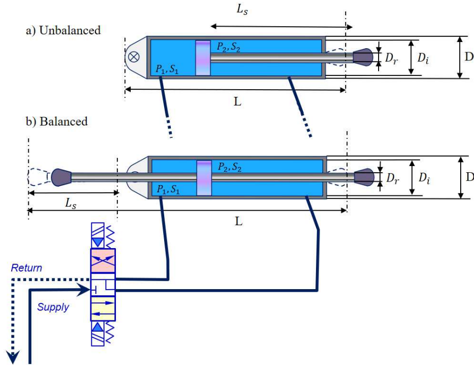
Fig. 2 Piston schematics for unbalanced and balanced actuators
