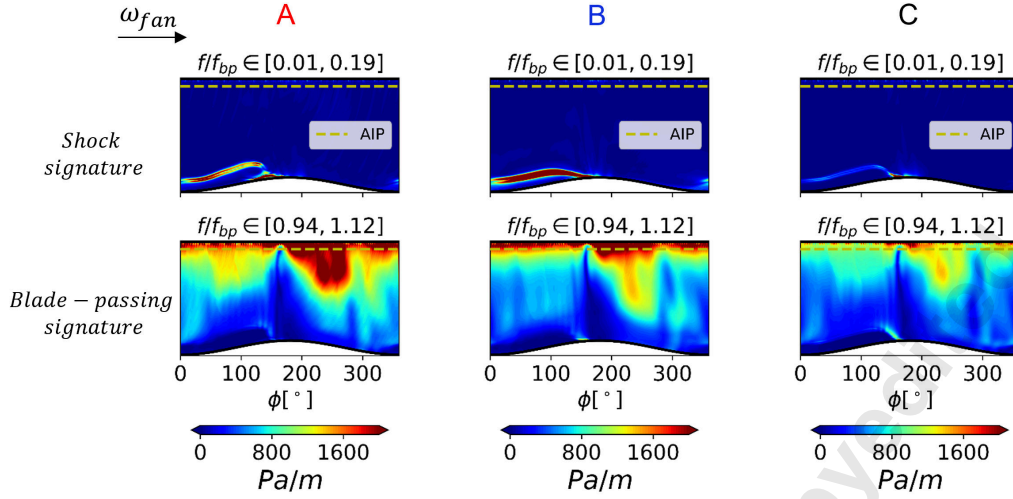
Fig. 18 Banded Fourier spectra of the fluctuations of the axial static pressure gradient on the intake surface. URANS-TRF simulations at V_{wind} = V_{wind,c}
