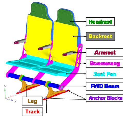
Figure 1 Nomenclature of “Sleep Seat” (Courtesy BlueSky) [1]
