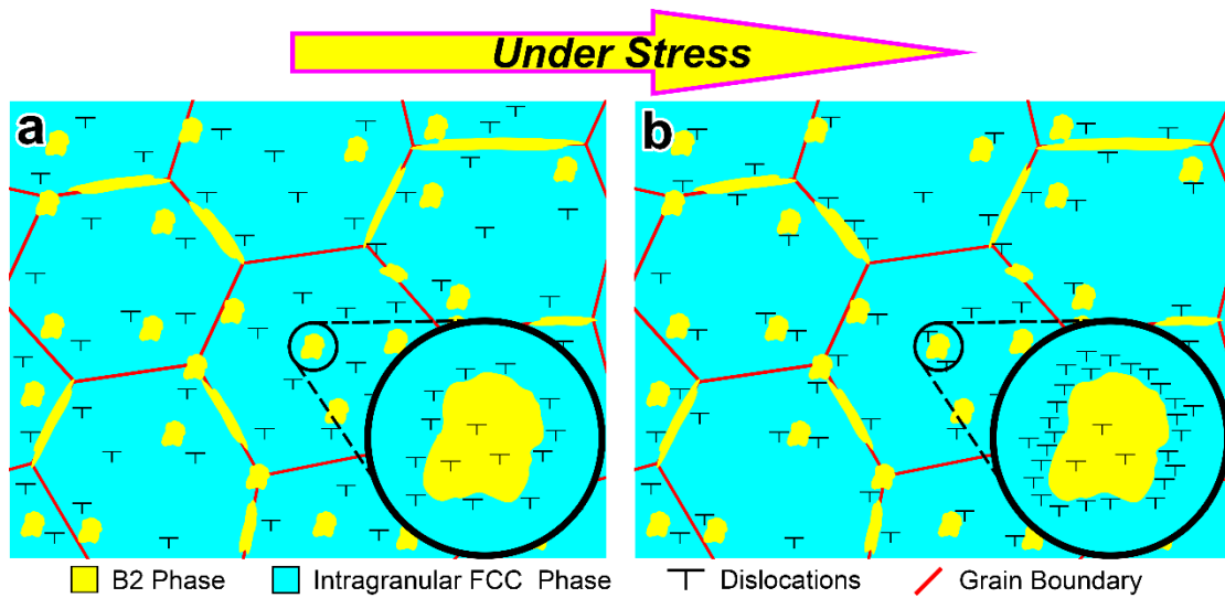
Fig. 12 Diagram of the strain-hardening mechanism of LMD-ed FeCoCrNiAl 0.5 HEA:
