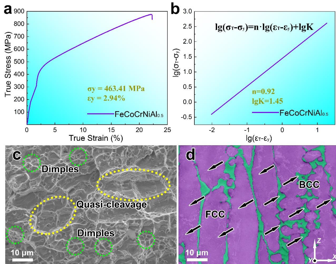
Fig. 2 Mechanical properties of LMD-ed FeCoCrNiAl 0.5 : (a) true stress-strain curves and (b) fitted work hardening exponents (linear function images); microstructure: (c) SEM image of tensile fracture and (d) EBSD phase distribution image.
