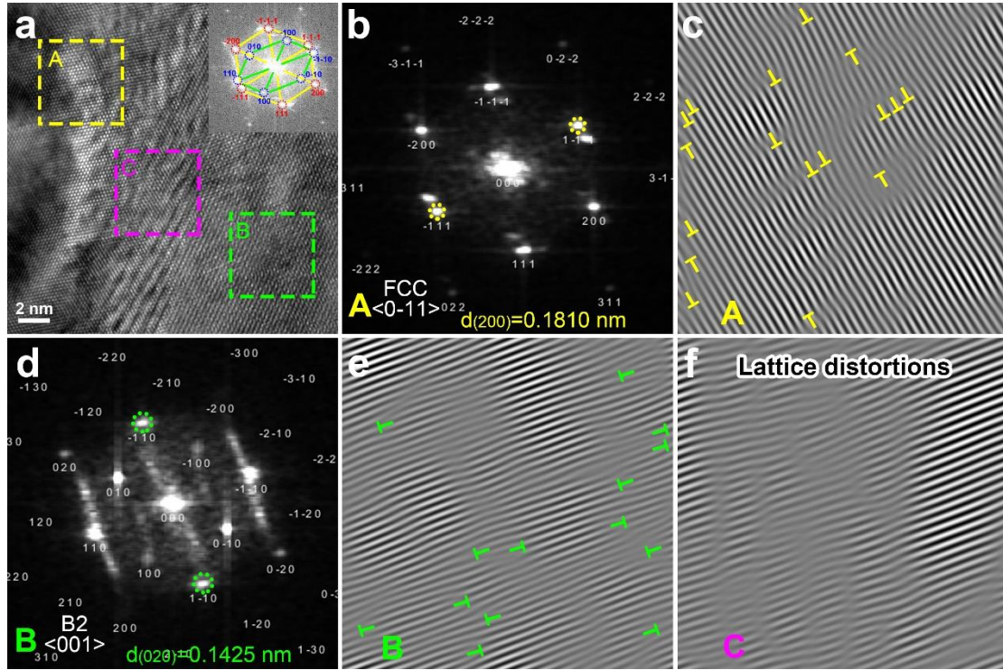
Fig. 5 (a) HR-TEM image with FFT pattern of FCC-B2 phase boundary; (b) FFT pattern of FCC-zone 'A' in (a); (c) IFFT lattice fringe of FCC-zone 'A' based on the marked spots in (b); (d) FFT patterns of B2-zone 'B' in (a); (e) IFFT lattice fringe of B2-zone 'B' based on the marked spots in (d); IFFT lattice fringe of boundary-zone 'C' in (a).
