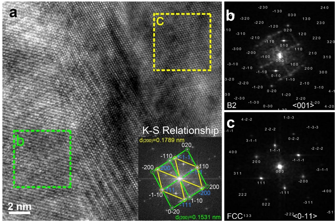
Fig. 6 (a) HR-TEM image of FCC-B2 phase boundary with FFT pattern; (b) FFT pattern of B2-zone in (a); (c) FFT pattern of FCC-zone in (a).
