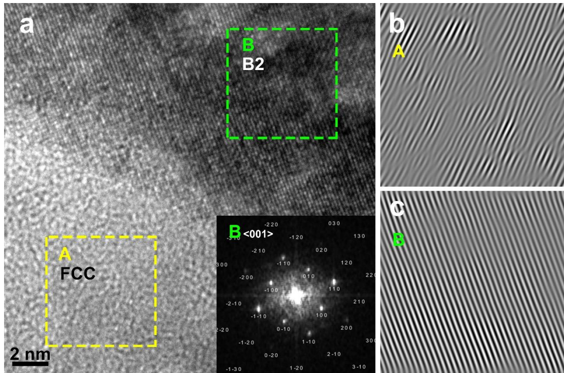
Fig. 7 (a) HR-TEM image of FCC-B2 phase boundary with FFT pattern of B2-zone 'B'; (b) IFFT lattice fringe of FCC-zone 'A' in (a); (c) IFFT lattice fringe of B2-zone 'B' in (a).
