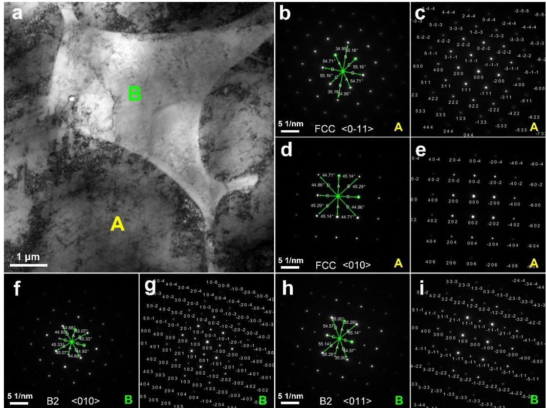
Fig. 3 (a) TEM image of LMD-ed FeCoCrNiAl 0.5 HEA; (b-e) SAED patterns of zone ‘A’ in (a); (f-i) SAED patterns of zone ‘B’ in (a).
