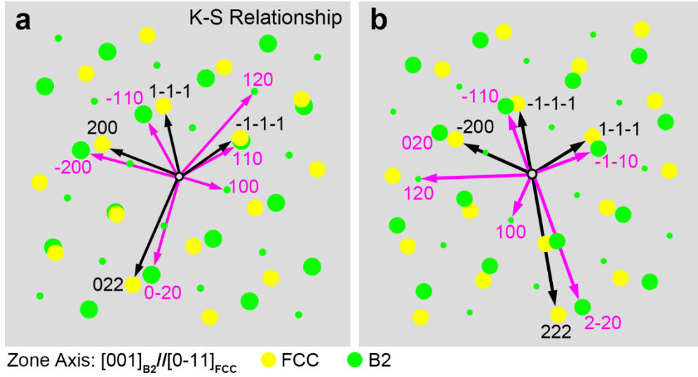
Fig. 10 Simulated diffraction pattern of phase boundary at the zone axis
