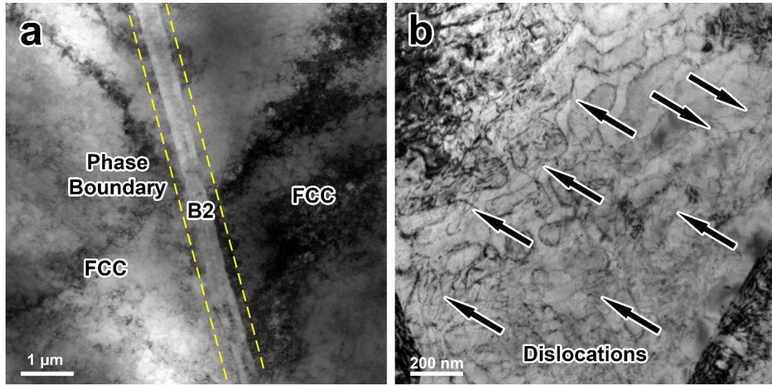
Fig. 8 (a) TEM image of slender B2-zone and phase boundary; (b) TEM of dislocation tangle at the grain boundary.
