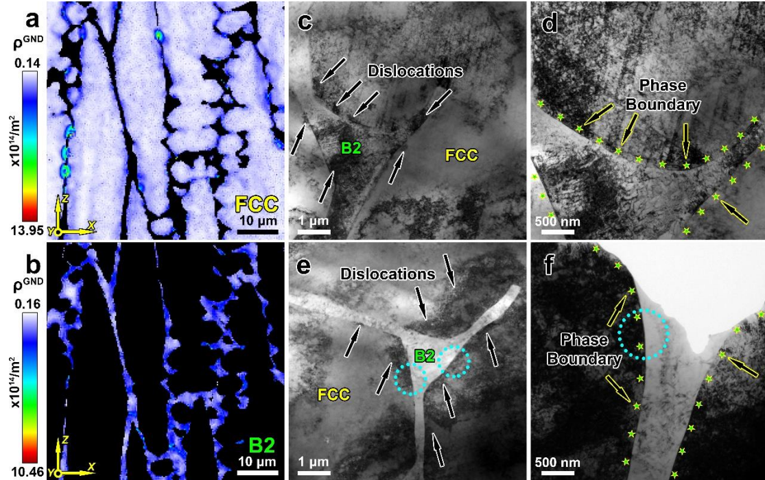
Fig. 4 (a) Distribution of GND density in FCC phase zones; (b) distribution of GND density in B2 phase zones; (c-f) TEM image showing dislocations distributions and phase boundaries: (d) is the local magnification of (c), (f) is the local magnification of (e).
