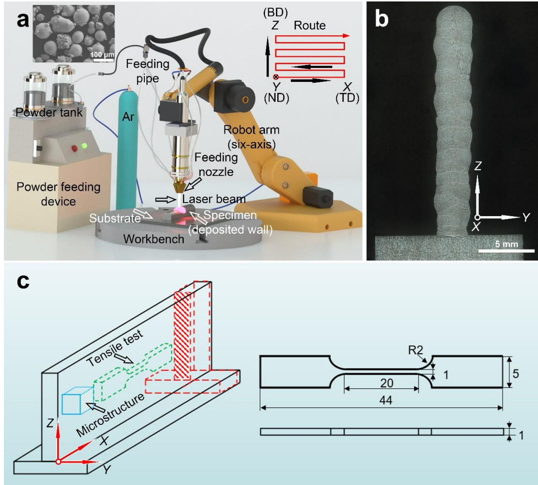
Fig. 1 (a) Schematic diagram of LMD system and processing route; (b) morphology of cross section (Y-Z plane); (c) schematic diagram of sampling.
