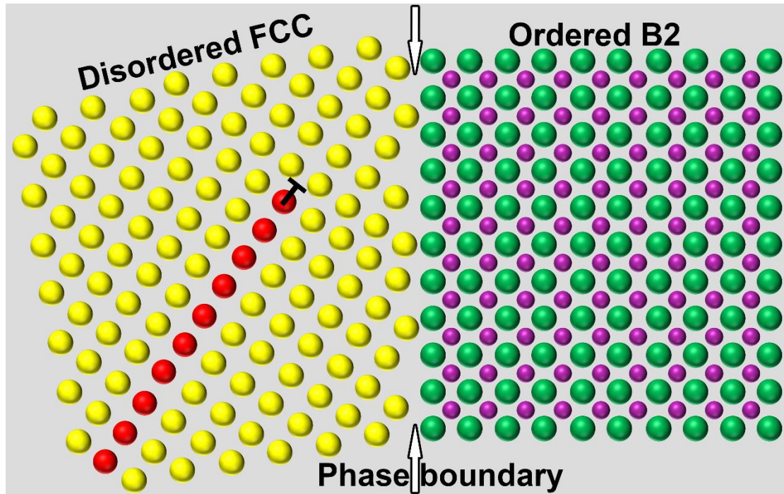
Fig. 11 Atomic diagram at phase boundary.
