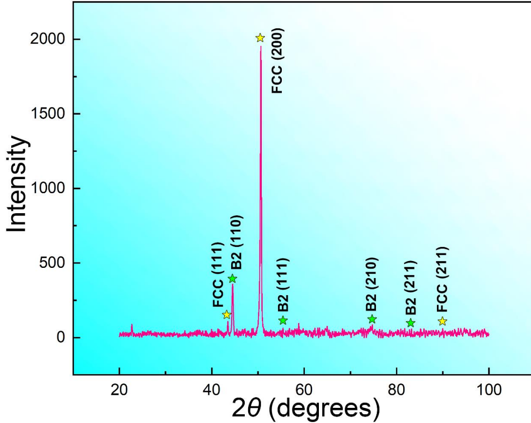
Fig. 9 XRD pattern of LMD-ed FeCoCrNiAl 0.5 HEA.
