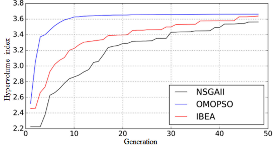
Fig. 5 Optimisation history of the NSGAI, OMOPSO and IBEA algorithms applied to Zitzler-Deb-Thiele's function N [33].
