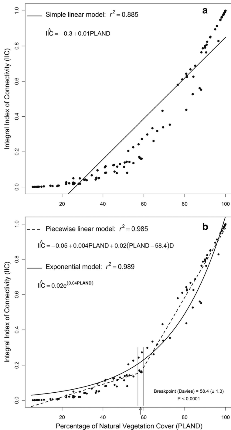
Fig. 3 Relationship between the percentage of natural vegetation (PLAND) and integral index of connectivity (IIC). Straight line represents the estimated regression equation based on a simple linear model (a). The dashed lines represent a piecewise linear regression model (where C = 58.4 is the threshold point and D is a dummy variable with D = 0 for C < 58.4 and D = 1 for C \geq 1 ), and the vertical arrows represents the breakpoints identified using the Davies test (with \pm se ) (b)
