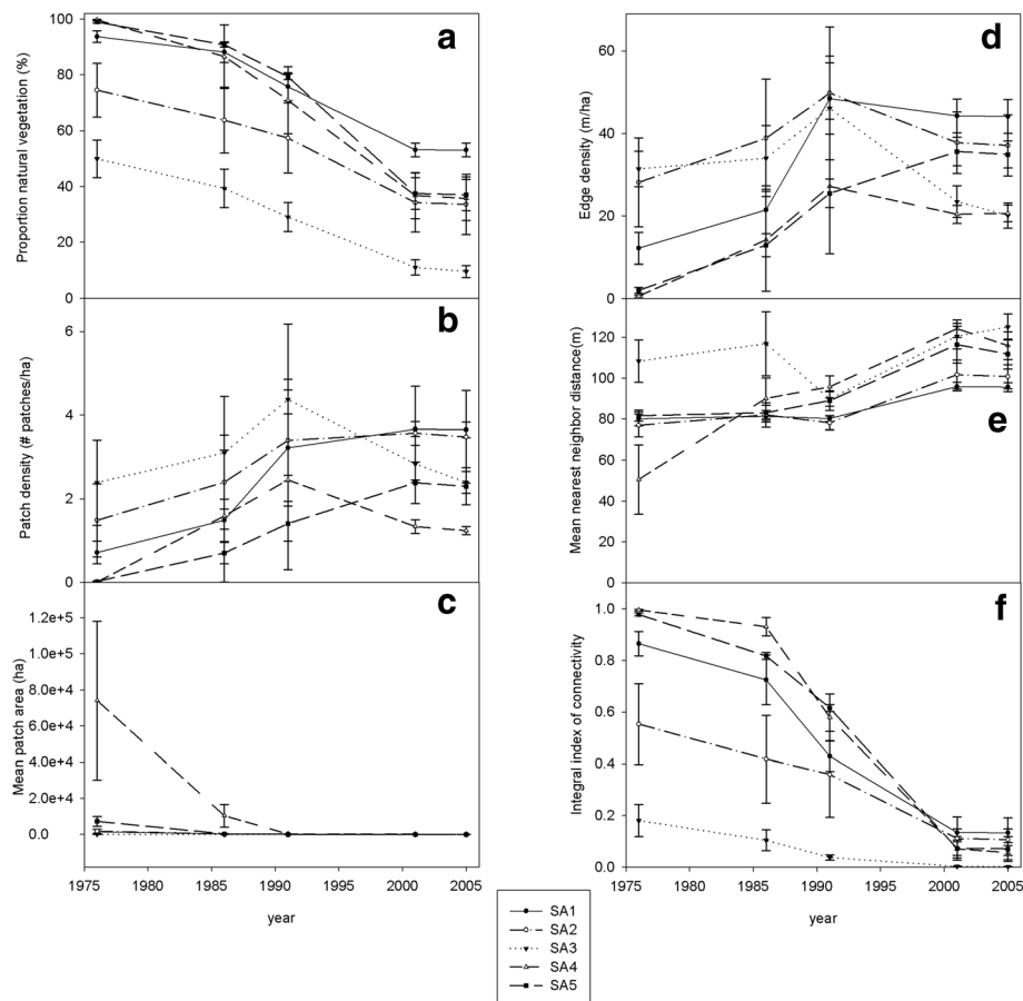
Fig. 2 Landscape metrics describing fragmentation and connectivity in five deforestation patterns in the lowland tropical forests in Bolivia: proportion of natural vegetation (a), patch density (b), mean patch area (c), edge density (d), mean nearest neighbour distance (e) and connectivity (f). The five deforestation patterns are the Chapare region (SA1), northwest colonization zone (SA2), the Santa Cruz integrated zone (SA3), the southern expansion zone (SA4) and the northern expansion zone (SA5)
