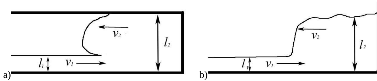
Figure.1 a) Constrained flow schematic b) Unconstrained flow schematic
