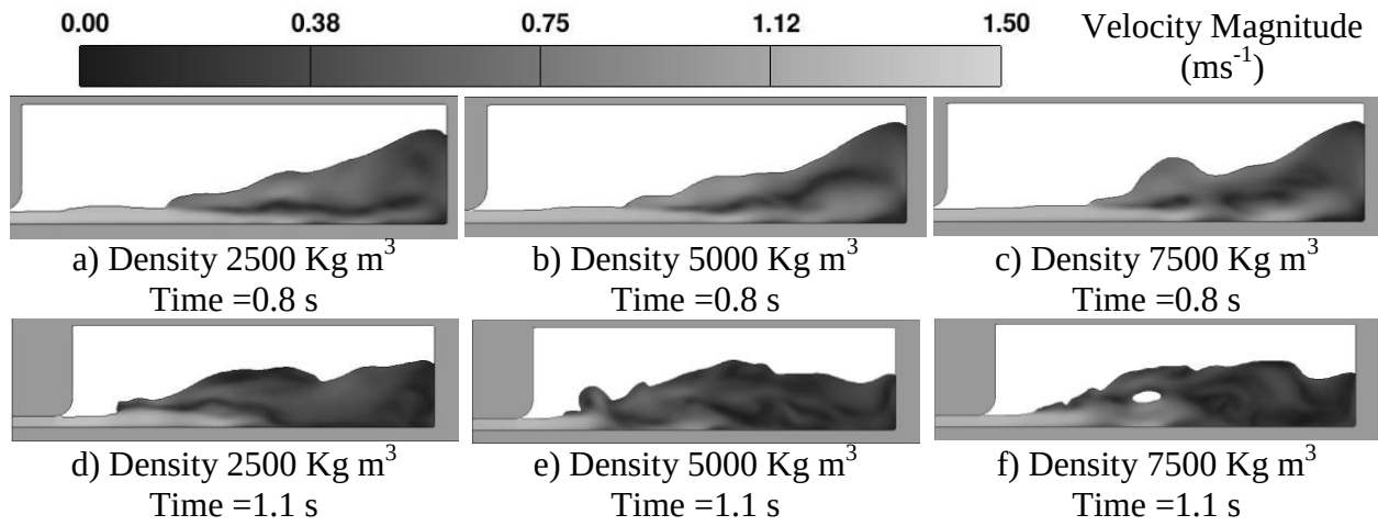
Figure 11. Comparison of wave heights for three materials of different densities. Surface tension (1 Nm -1 ) and viscosity (0.001 Pa s) remain the same. Fluid velocity is 1.18ms -1
