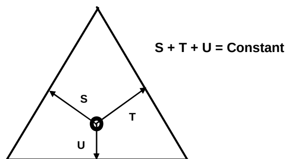
Figure 5. Equilateral triangle: perpendiculars from a point
