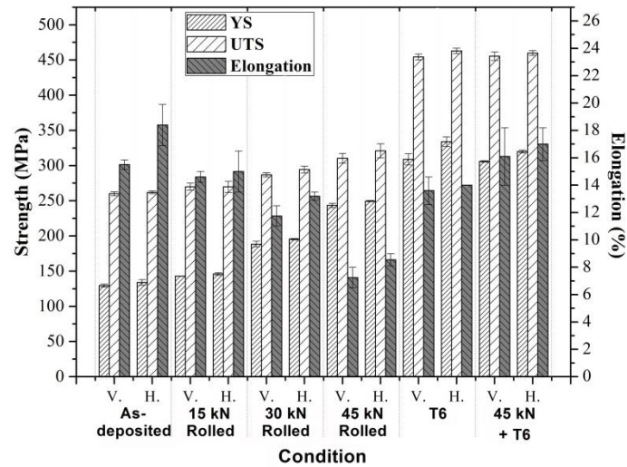
Fig. 5. Tensile properties for the as-deposited, inter-layer rolled and heat treated WAAM 2219
