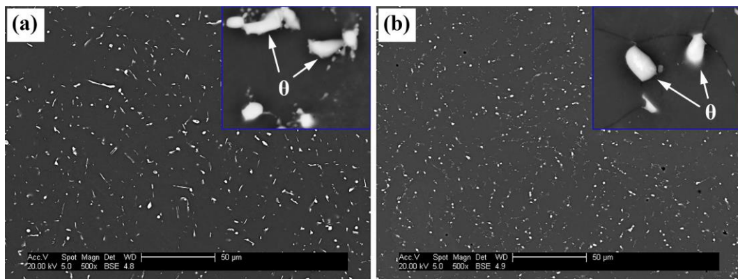
Fig. 11. Scanning electron micrographs for the WAAM 2219 alloys (a) after-deposition T6 treated and (b) 45 kN rolled + T6 treated.
