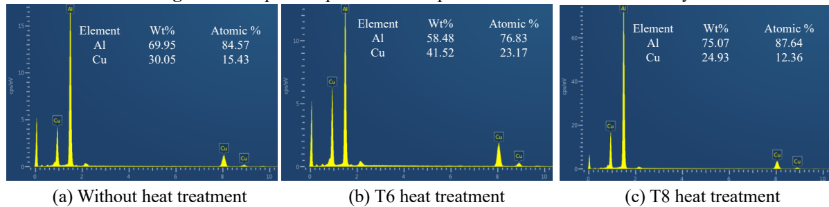
Figure 4 Energy dispersive spectrometry (EDS) analysis of precipitates
