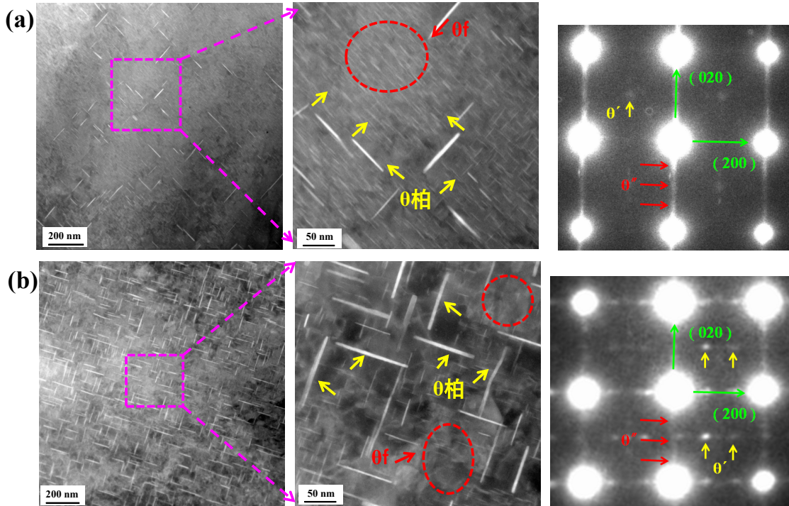
Figure 8 Precipitates distribution of : (a) T6 heat treatment and (b) T8 heat treatment
