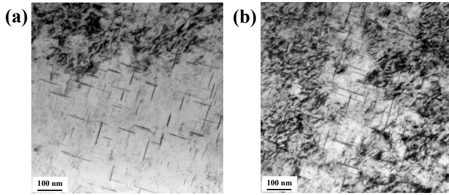
Figure 7 TEM micrographs of : (a) T6 heat treatment and (b) T8 heat treatment
