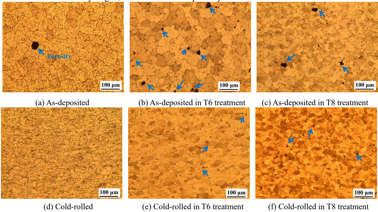
Figure 2 Microstructure variation with different heat treatments
