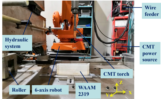
Figure 1 Experimental set up of hybrid WAAM deposition and rolling system
