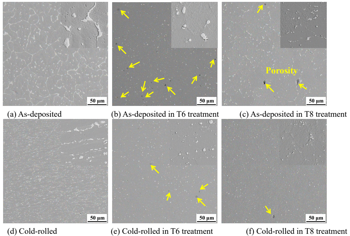
Figure 3 Precipitation phases in as-deposited and cold-rolled 2219 alloy
