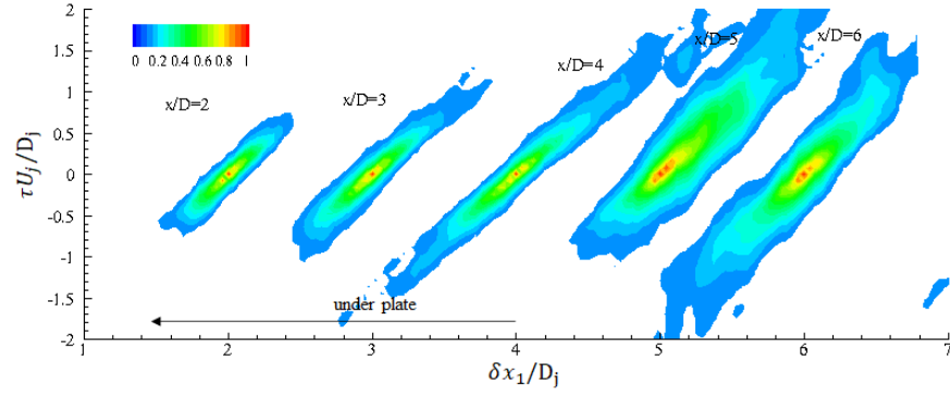
(c) Installed jet, H/D=0.67
