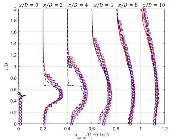
(b) axial velocity fluctuations
