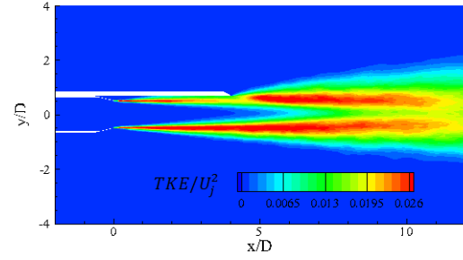
(f) Turbulent kinetic energy in the isolated jet ( H/D=0.67 )
