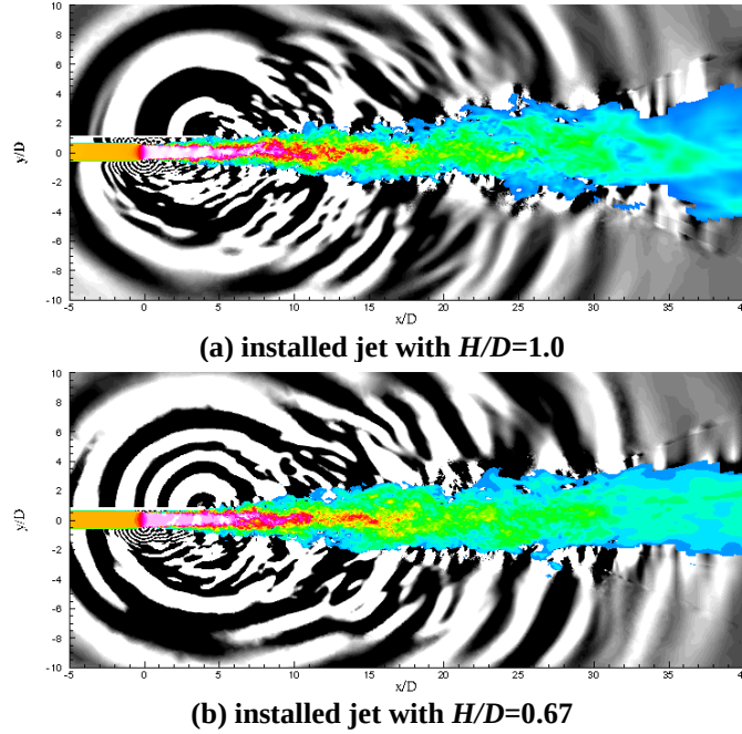
Figure 2 Flow and acoustics of two installed jets: axial velocity in colour contours and pressure time derivatives in grey-scale contours
