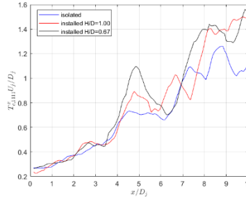
(b) Time scales
