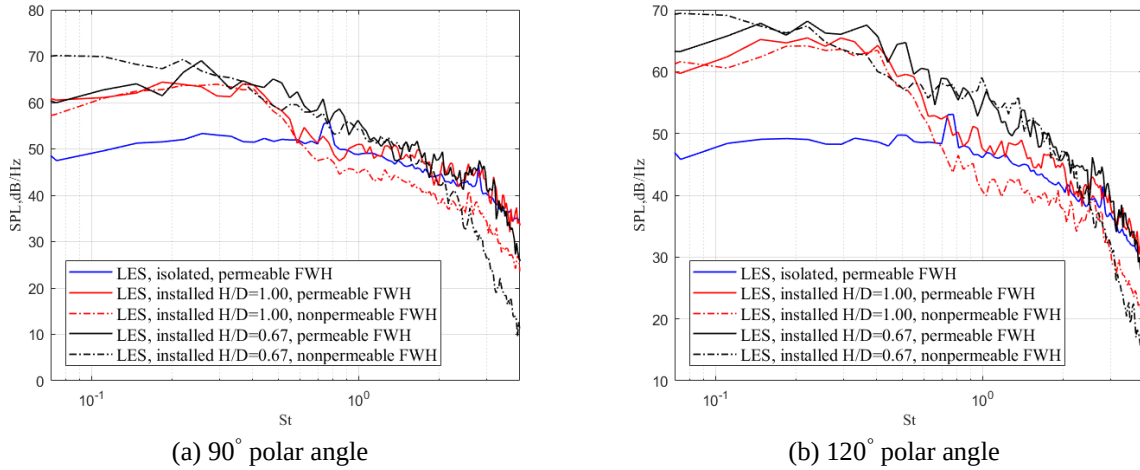
Figure 10 Comparison of far-field noise prediction from permeable FW-H surface around the jet and nonpermeable FW-H surface on the plate at 90^\circ and 120^\circ polar angles
