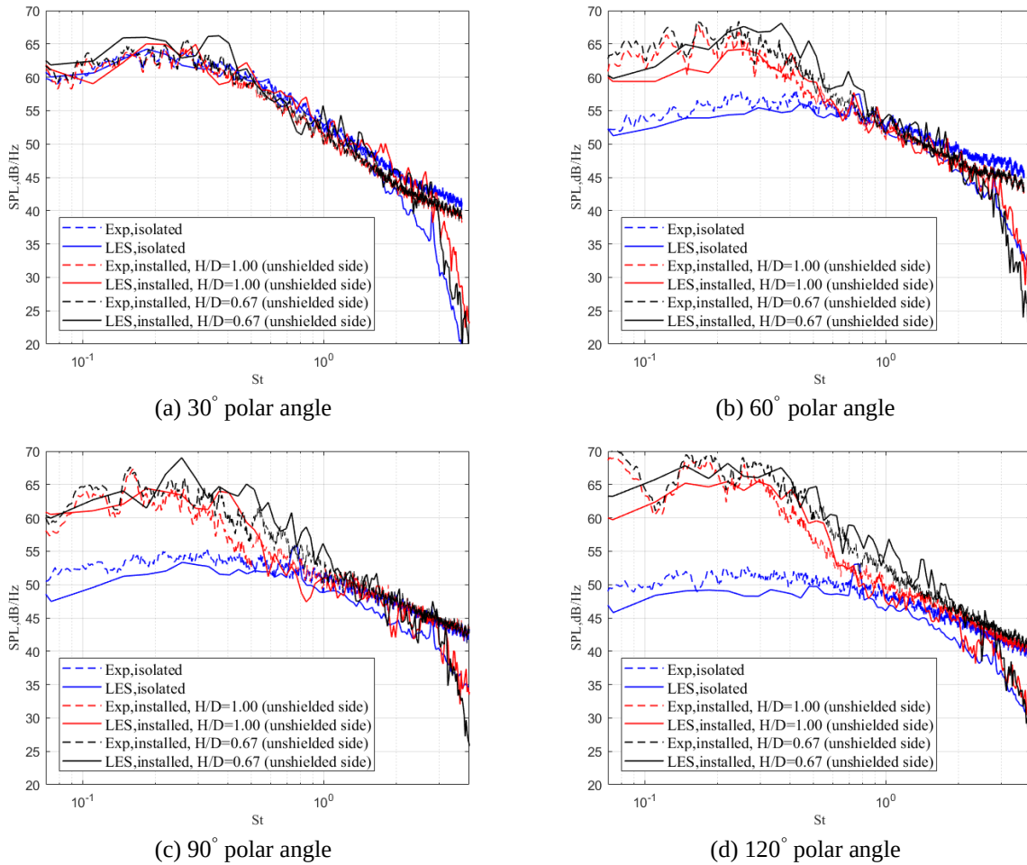
Figure 5 Far-field noise with four polar angles ( 30^\circ , 60^\circ , 90^\circ and 120^\circ ) from the downstream direction on the unshielded side
