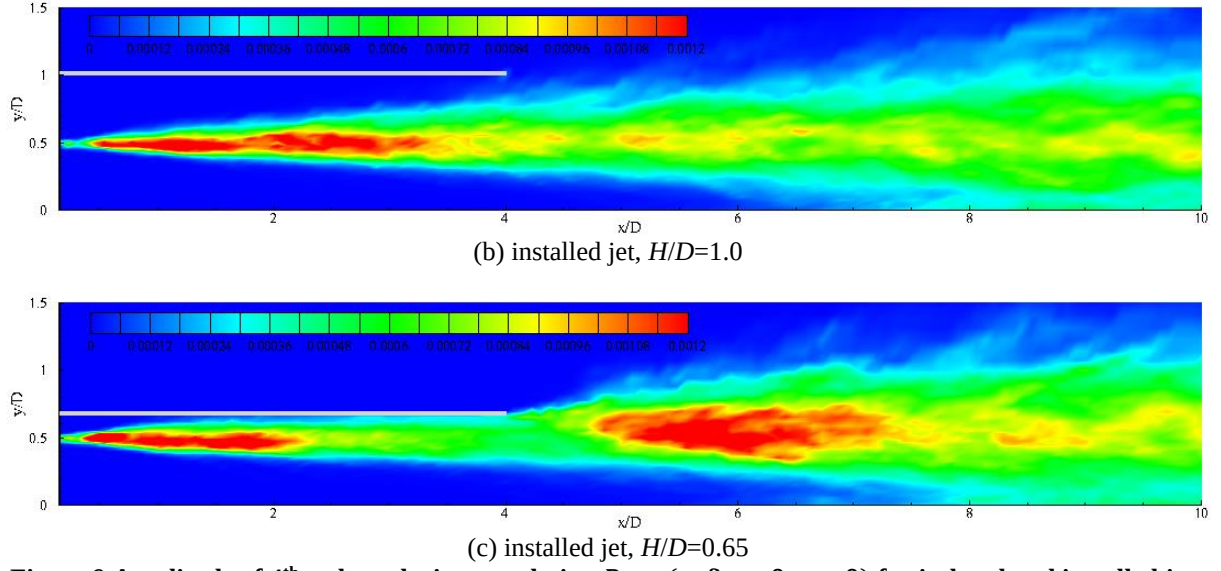
Figure 9 Amplitude of 4 th order velocity correlation R_{1111}(x; \delta x = 0, \tau = 0) for isolated and installed jets
