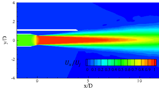
(c) Axial velocity in the installed jet ( H/D=1 )
