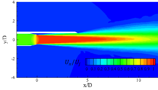
(e) Axial velocity in the installed jet ( H/D=0.67 )
