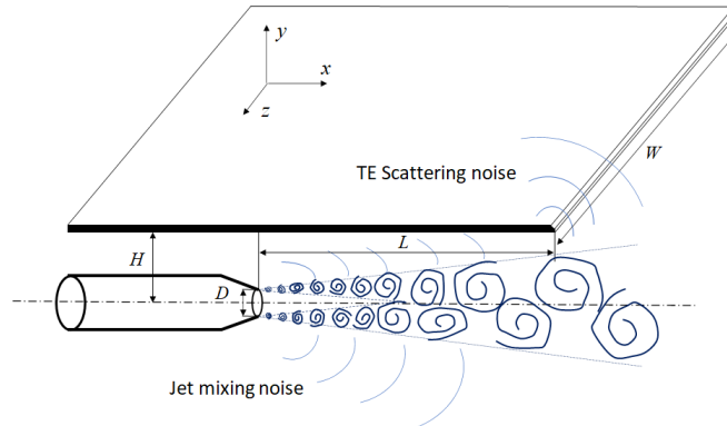
Figure 1 Schematic of canonical installed jets
