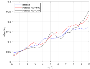
(a) Length scales
