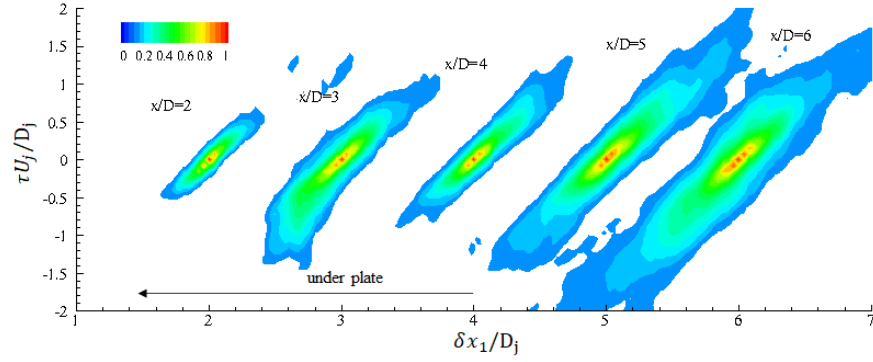
(b) Installed jet, H/D=1.00
