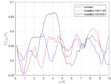
(c) Convection velocity
