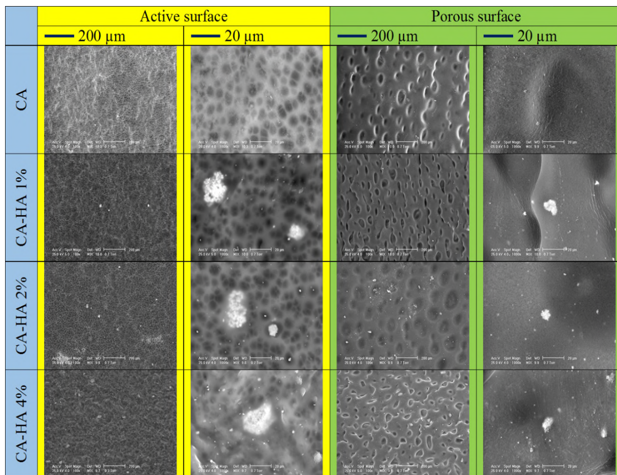
Fig. 1 SEM micrographs of synthesized membranes
