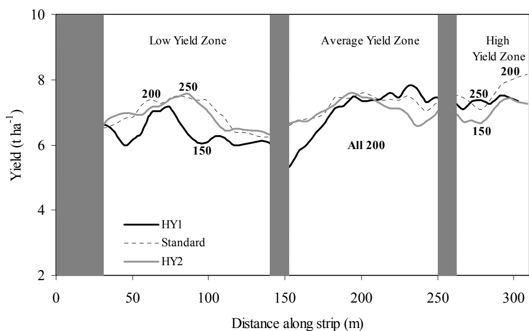
Fig. 14. Combine Yield ( t\ ha^{-1} ) of the Historic Yield (HY) strategy treatment strips in Twelve Acres in 1997/98. Shaded area represents lead-in time of combine harvester. Numbers in bold ( 150, 200, 250 ) are the N application rate in kg\ N\ ha^{-1} . —, HY1; ---, Standard; —, HY2
