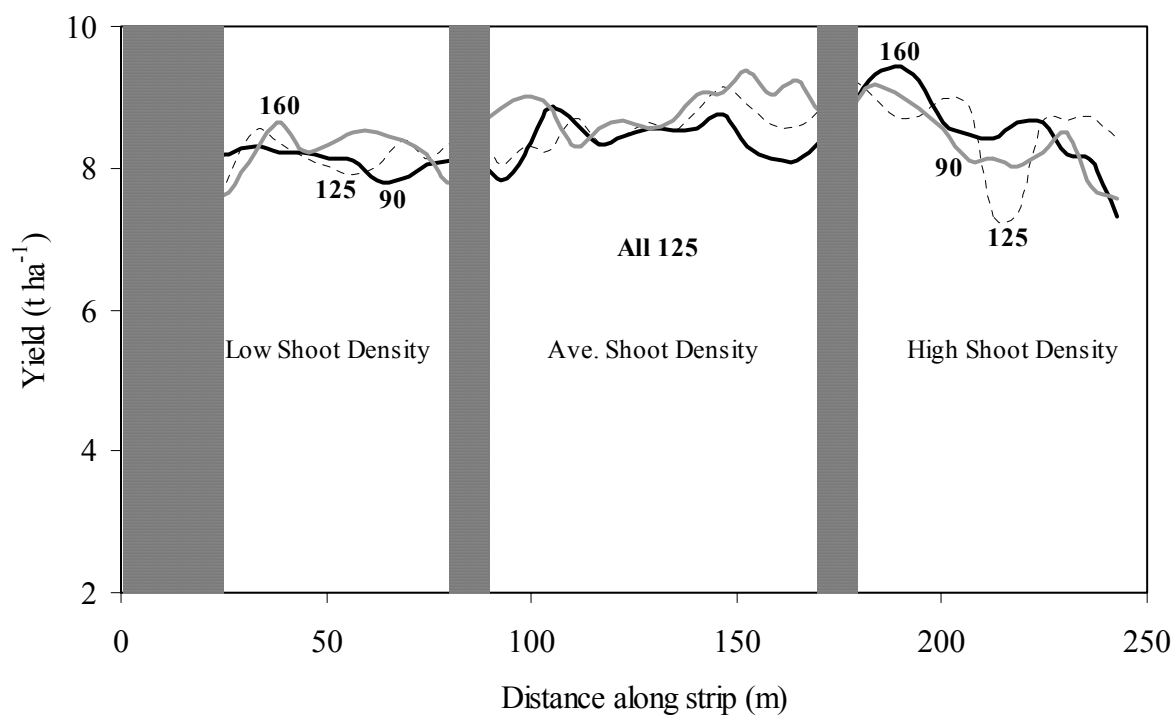
Fig. 17. Combine Yield ( t\ ha^{-1} ) of the Shoot Density (SD) strategy treatment strips in Far Sweetbrier in 1997/98. Shaded area represents lead-in time of combine harvester. Numbers in bold ( 90 , 125 , 160 ) are the N application rate in kg\ N\ ha^{-1} . —, SD1; ----, Standard; —, SD2
