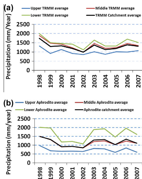
Fig. 3. Comparison of annual (a) APHRODITE and (b) TRMM precipitation data at the sub-catchment scale.
