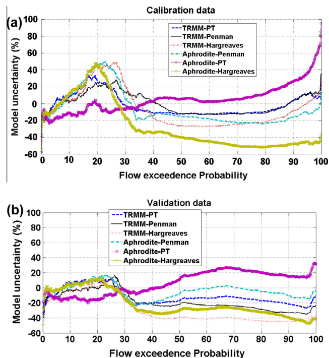
Fig. 8. (a–b) Model uncertainty (as given by the percentage difference between simulated and observed discharge) along the flow exceedance curves showing associated uncertainties in six hydrological modelling setups under the calibration (2000–2004) and validation (2005–2008) phases.
