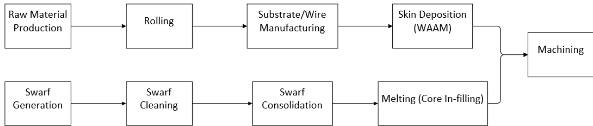
Figure 3 WAAM-SI process map.
