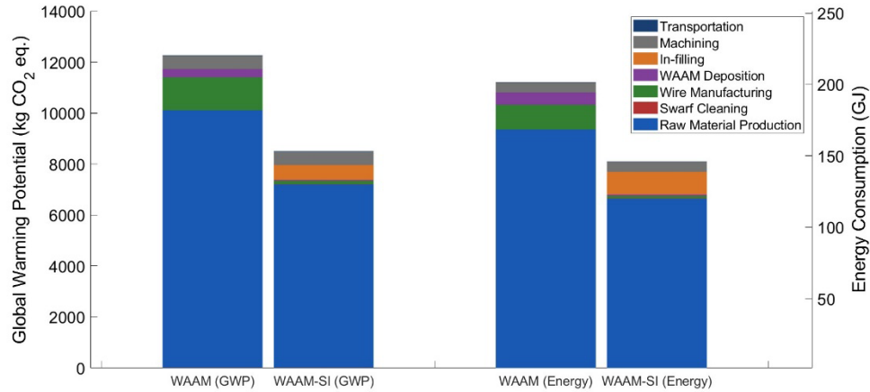
Figure 4 Global Warming Potential (kg CO 2 eq.) and Energy consumption (GJ) breakdown of Wire Arc Additive Manufacturing (WAAM) and Wire Arc Additive Manufacturing Solid Infill (WAAM-SI).
