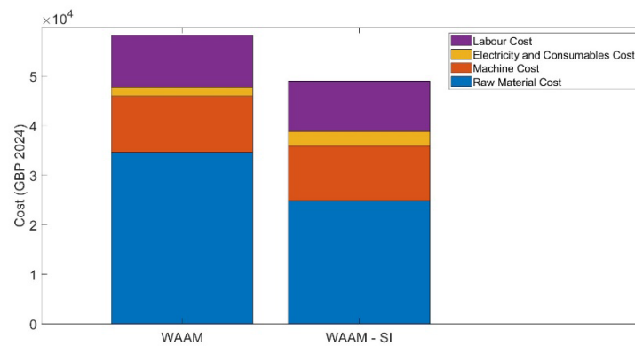
Figure 5 Cost breakdown of Wire Arc Additive Manufacturing (WAAM) and Wire Arc Additive Manufacturing Solid Infill (WAAM-SI).
