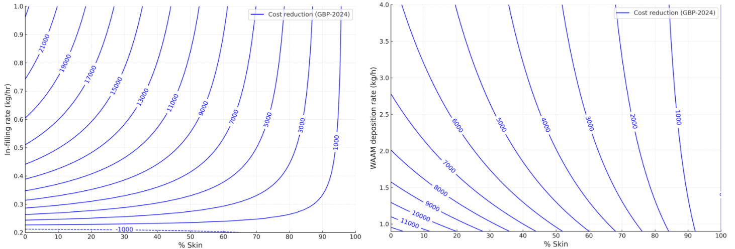
Figure 6 & 7 Cost reduction (GBP) of WAAM-Solid Infill (WAAM-SI) relative to WAAM as a function of skin percentage vs in-filling rate (Fig 6), and vs deposition rate (Fig 7), where 100% skin = WAAM baseline.
