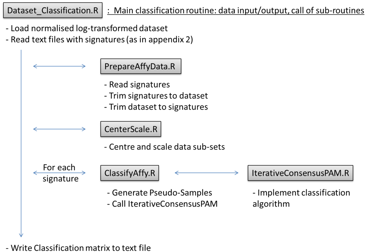
Figure 18: Implementation of classification in R
