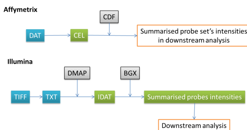
Figure 9: Affymetrix and Illumina source data files
