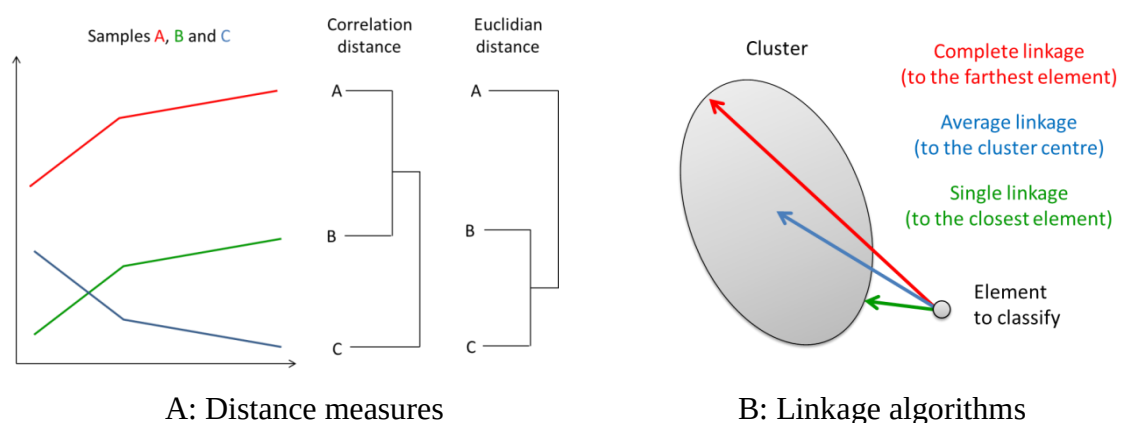
Figure 11: Effects of Distance Measure and Linkage Algorithms on Clustering
