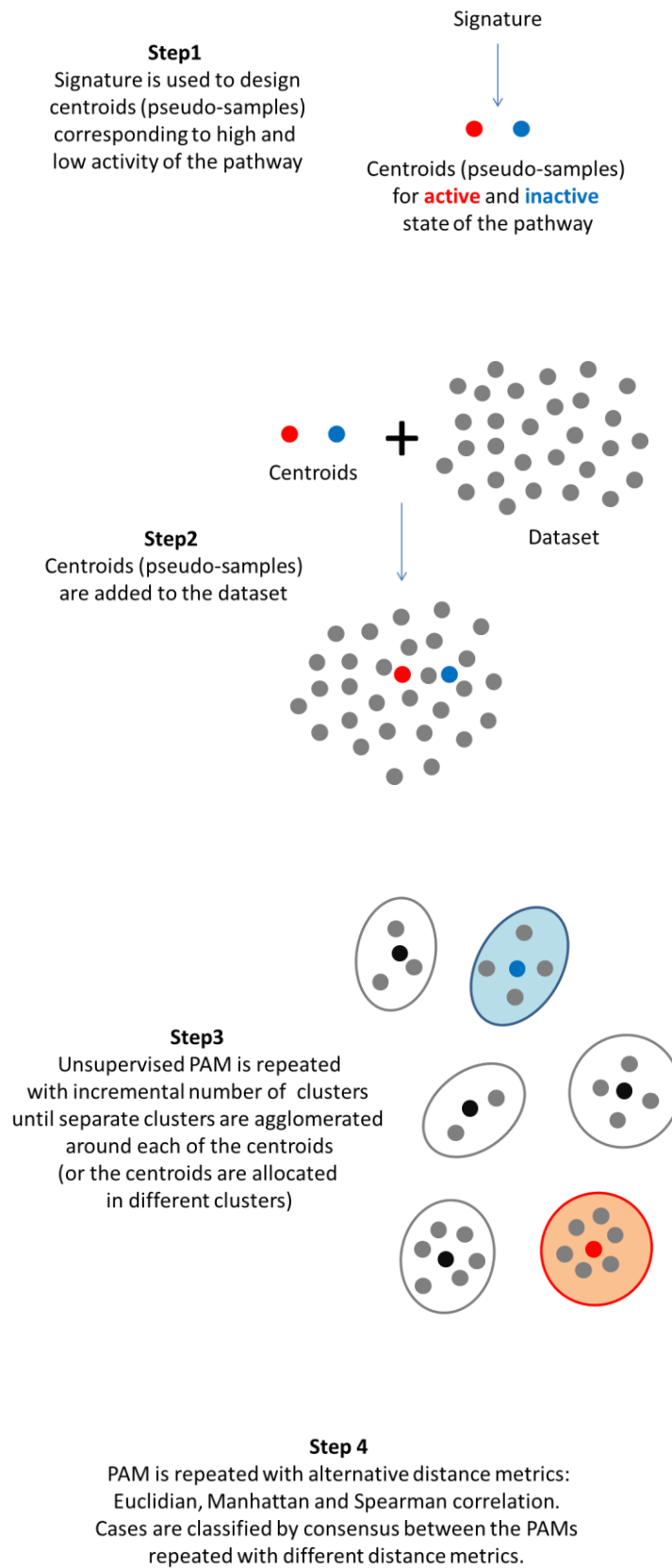
Figure 17: Classification algorithm: Iterative Consensus PAM
