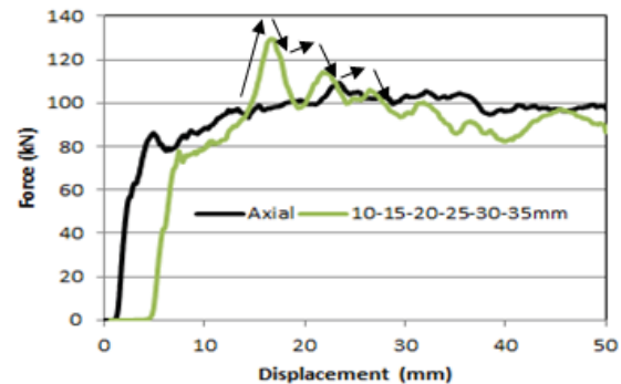
Fig. 5 Force displacement graph comparison between non-stitched absorber and 10-15-20-25-30-35 mm multi-stitched absorbers
