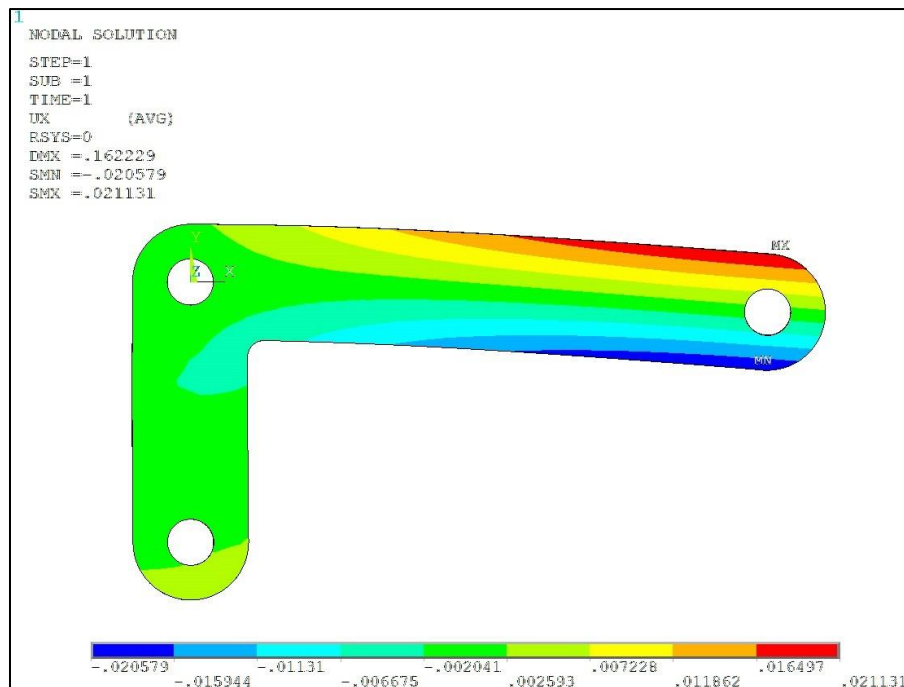
Figure 10. Displacement in the x-axis results for the solid bracket.
