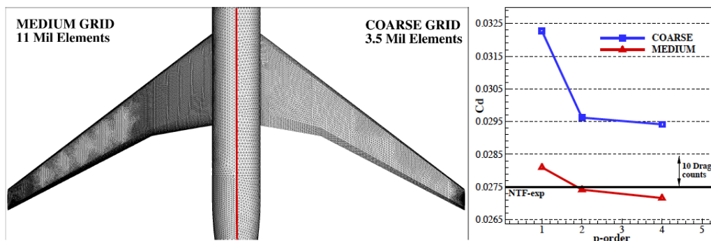
Figure 3: The RANS case: Mesh geometry and total drag coefficient
