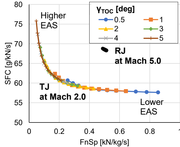
Figure IV-13: Relationship between Specific Net Thrust, FnSp, and Specific Fuel Consumption, SFC, for the turbojet powerplant at Mach 2.0 and the ramjet at Mach 5.0 for a range of \gamma_{\text{TOC}} and climb EAS.
