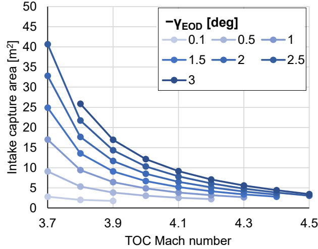
Figure IV-5: Intake area for a range of EOD angles of dive ( -\gamma_{EOD} ) and TOC Mach numbers.
