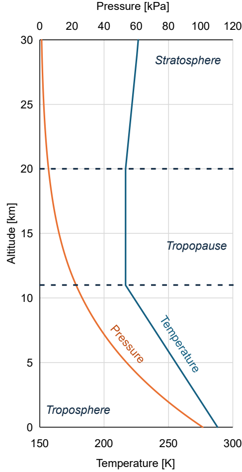
Figure IV-2: Values of pressure and temperature with altitude according to the International Standard Atmosphere model [26].
