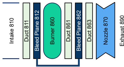
Figure III-2: Component models of the TBCC model: A) Single-spool turbojet with a turbine cooling bleed and an afterburner cooling jacket bleed. B) Ramjet model with combustor cooling bleed.
