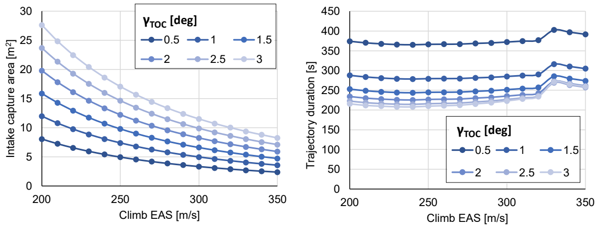
Figure IV-1. Left: Intake area as a function of both climb Equivalent Airspeed (EAS) and Top-of-Climb angle of climb ( \gamma_{\text{TOC}} ). Right: Trajectory duration as a function of both climb EAS and \gamma_{\text{TOC}} .
