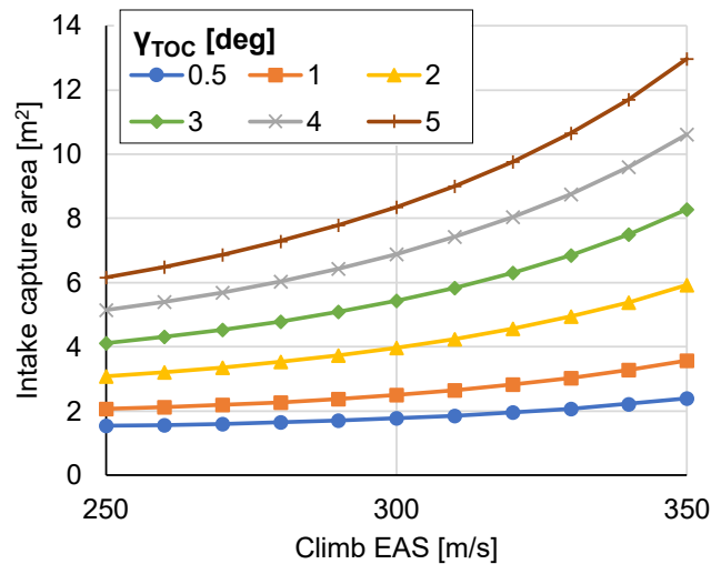
Figure IV-12: Intake area sized for a range of climb EAS and \gamma_{\text{TOC}} .
