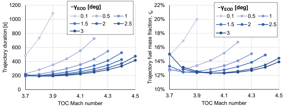
Figure IV-7: Left: Trajectory duration in terms of TOC Mach number and EOD angle of dive, -\gamma_{EOD} . Right: Trajectory fuel mass fraction, \zeta_t , in terms of TOC Mach number and -\gamma_{EOD} .
