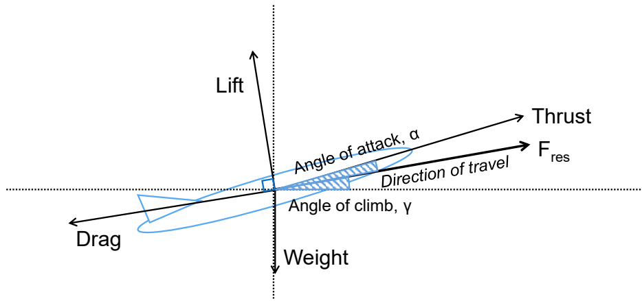
Figure III-6: Diagram of forces on lifting body in accelerating and climbing flight (not to scale).
