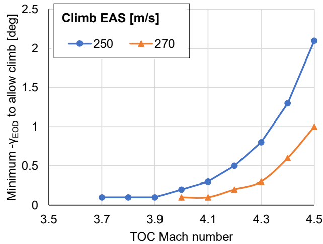
Figure IV-8: Minimum -\gamma_{EOD} required for powerplant to be able to sustain climb at a given TOC Mach number, for climb EAS of 250 and 270 m/s.
