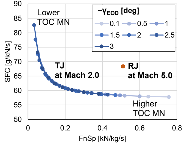
Figure IV-9: Relationship between Specific Net Thrust, FnSp, and Specific Fuel Consumption, SFC, for the turbojet powerplant at Mach 2.0 and the ramjet at Mach 5.0 for a range of -\gamma_{EOD} and TOC Mach number (MN).
