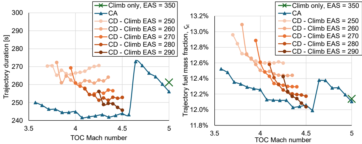
Figure IV-15. Left: Total trajectory duration, and Right: Trajectory fuel mass fraction, \zeta_t , for: the baseline constant-EAS climb (“Climb only”); climb-accelerate (“CA”) trajectories at a range of TOC Mach numbers; and climb-dive (“CD”) trajectories with a range of TOC Mach numbers and -\gamma_{EOD} ; all with the same intake area and same Mach 5.0 EAS of 350 m/s.
