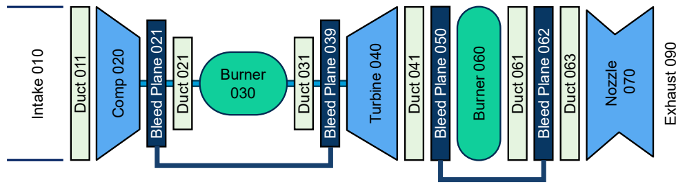
B) Ramjet model
