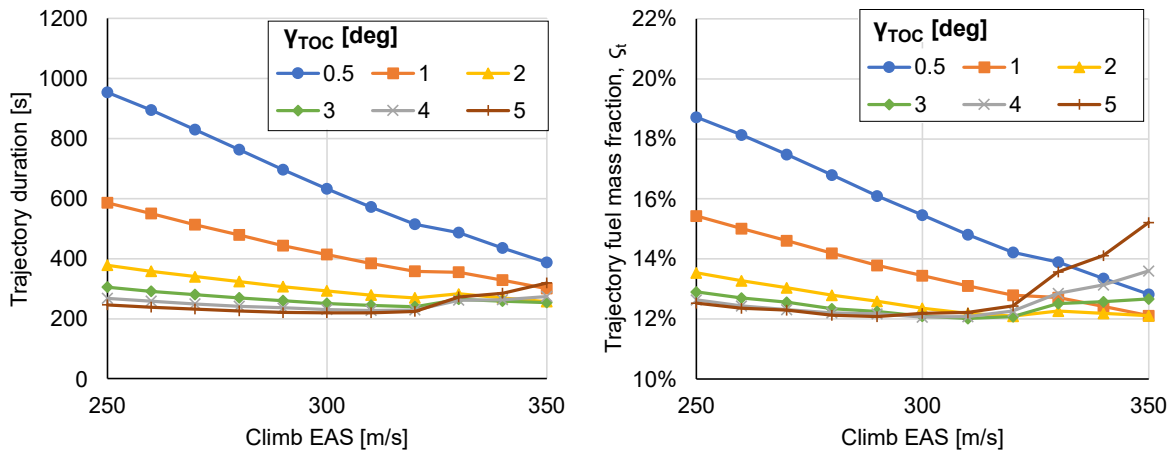
Figure IV-10. Left: Total trajectory duration as a function of both climb EAS and TOC angle of climb, \gamma_{TOC} . Right: Trajectory fuel mass fraction, \zeta_t , as a function of both climb EAS and \gamma_{TOC} .
