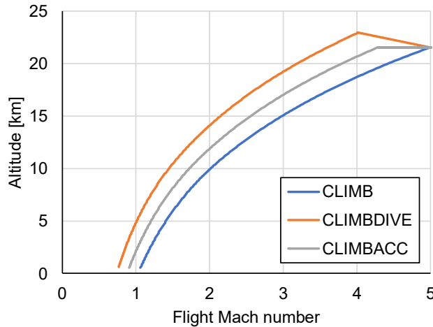
Figure III-7: Example constant-EAS climb, climb-dive, and climb-accelerate trajectories.
