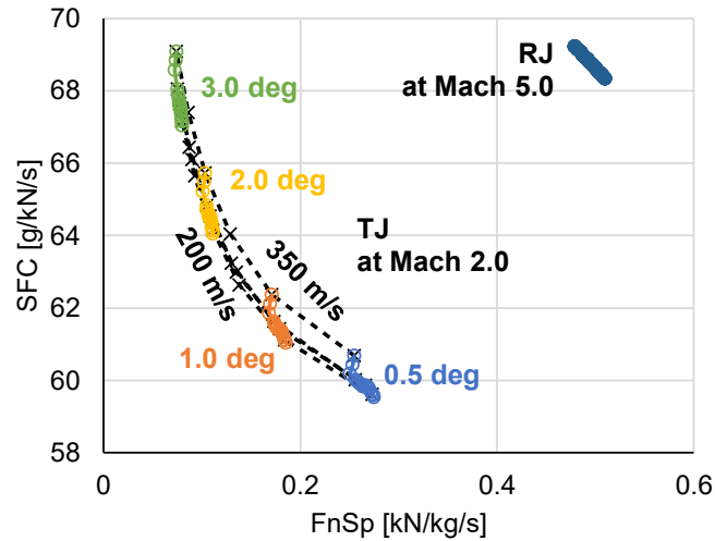
Figure IV-4: Relationship between Specific Net Thrust, FnSp, and Specific Fuel Consumption, SFC, for the turbojet powerplant at Mach 2.0 and the ramjet at Mach 5.0 for a range of \gamma_{TOC} and climb EAS.
