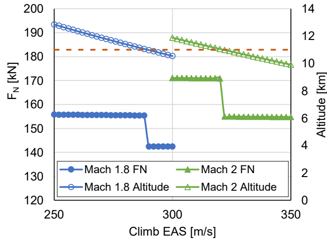
Figure IV-3: Net thrust, F_N , for 5 degree climb and altitude at Mach 1.8 and 2.0, for a range of climb EAS. For both Mach numbers, there is a step change in the thrust at 11 km.
