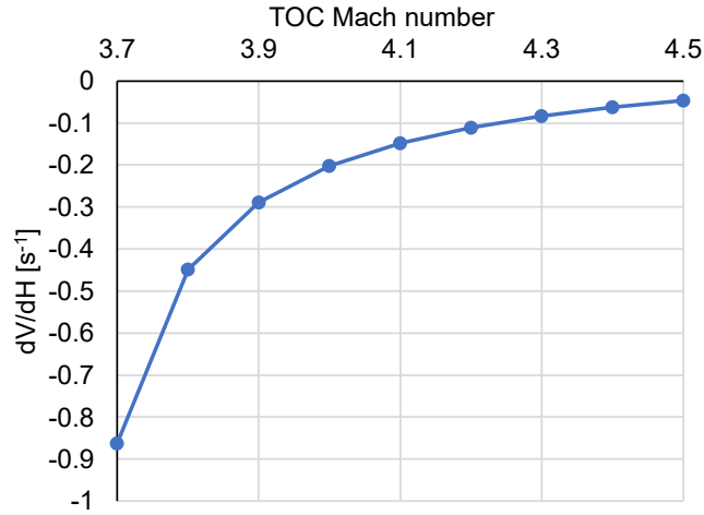
Figure IV-6: Change in velocity with altitude for dives from various TOC Mach numbers at 250 m/s EAS to Mach 5.0 at 350 m/s EAS.
