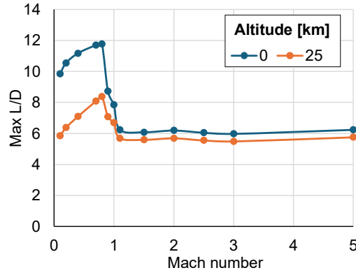
Figure III-5: Maximum L/D data for an aircraft analogous to the SR-71, with simplified geometry.
