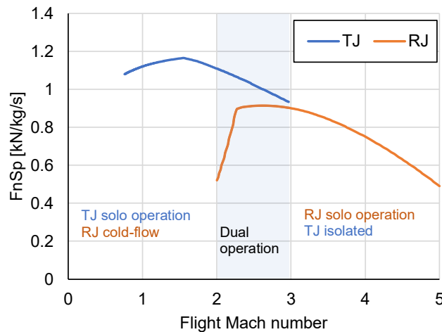
Figure III-3: Specific Net Thrust, FnSp, for the turbojet (TJ) and ramjet (RJ) powerplants in a climb. The FnSp of the ramjet increases sharply from Mach 2.0-2.3 as the ramjet throttles up to maintain a climb angle.
