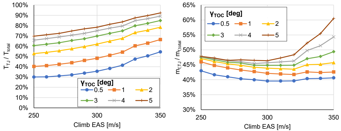
Figure IV-11. Left: Proportion of trajectory duration with the turbojet powerplant active ( T_{\text{TJ}}/T_{\text{total}} ), as a function of both climb EAS and \gamma_{\text{TOC}} . Right: Proportion of total trajectory fuel consumed by TJ ( m_{f,\text{TJ}}/m_{f,\text{total}} ), as a function of both climb EAS and \gamma_{\text{TOC}} .
