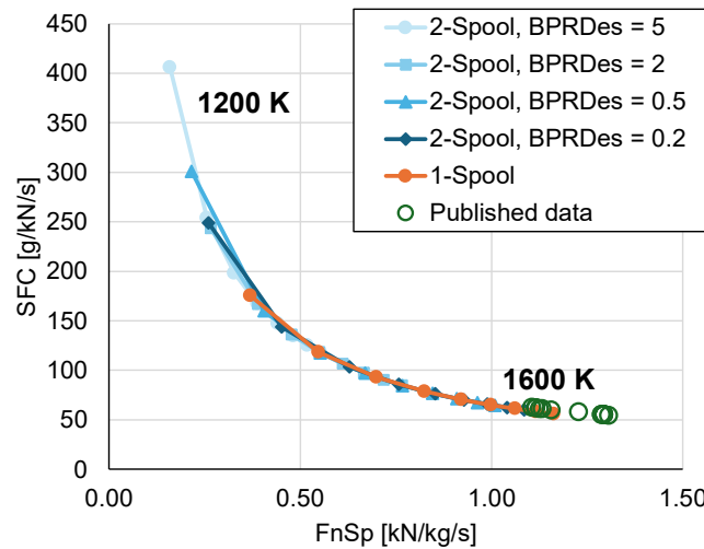
Figure III-4: Plot of SFC against FnSp for afterburning 1- and 2-spool engines with design TET from 1200 to 1600 K at SLS.
