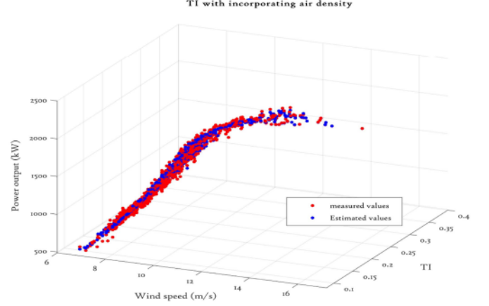
Fig. 5. GP power curve incorporating turbulence intensity.
