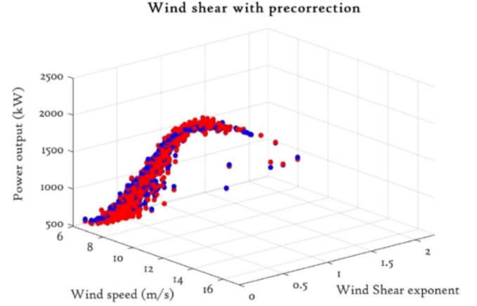
Fig. 8. GP power curve incorporating wind shear with pre-correction [red: measured, blue: estimated].
