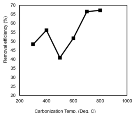
Figure 4: Plot of carbonization temp vs. removal efficiency.
