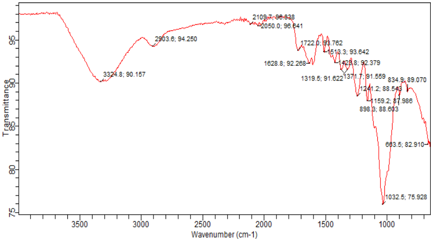
Figure 1: FTIR spectra of raw crabshell.
