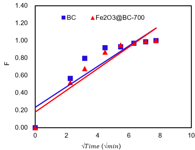
Figure 13: Plot of homogenous solid diffusion model.
