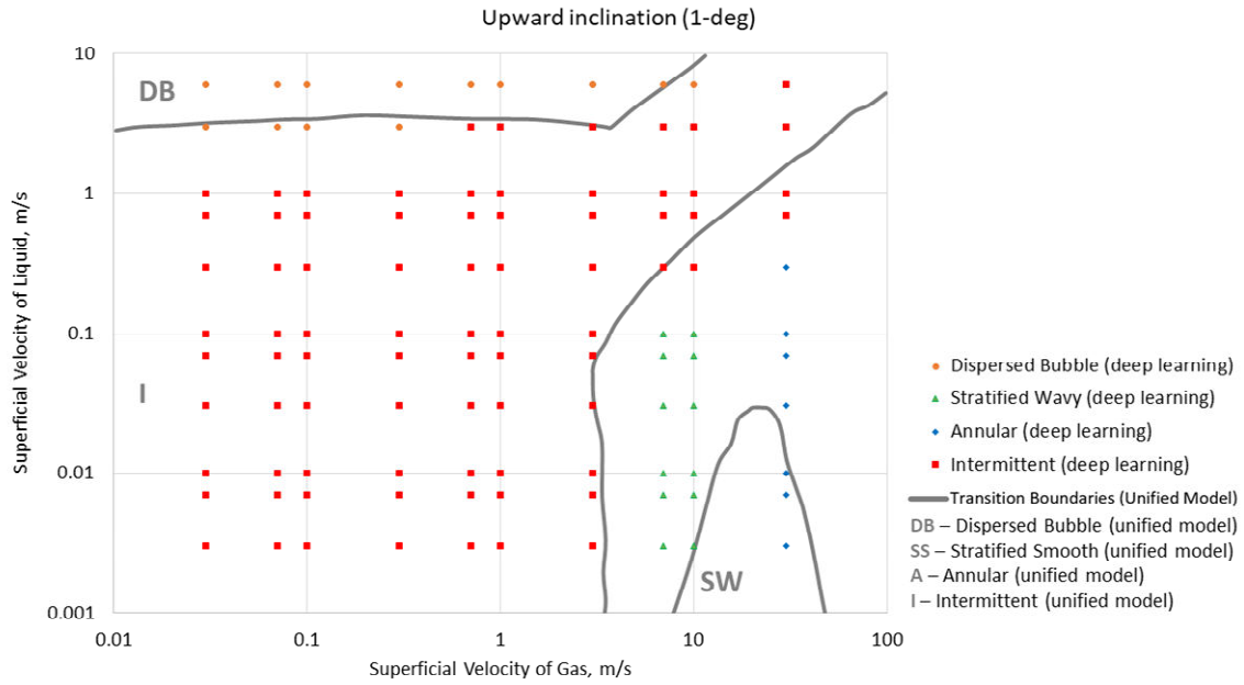
Fig. 7 – Comparisons of flow regime maps generated by deep learning model (dotted points) and unified model (full lines) for two-phase flow in upward inclined ( 1^\circ ) pipe.
