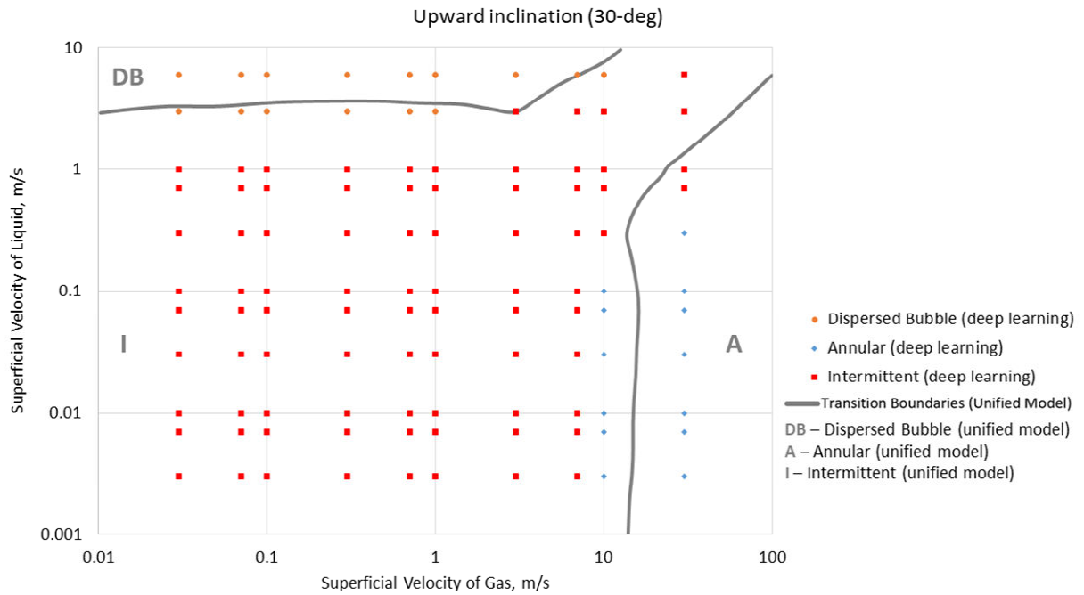
Fig. 8 – Comparisons of flow regime maps generated by deep learning model (dotted points) and unified model (full lines) for two-phase flow in upward inclined ( 30^\circ ) pipe.
