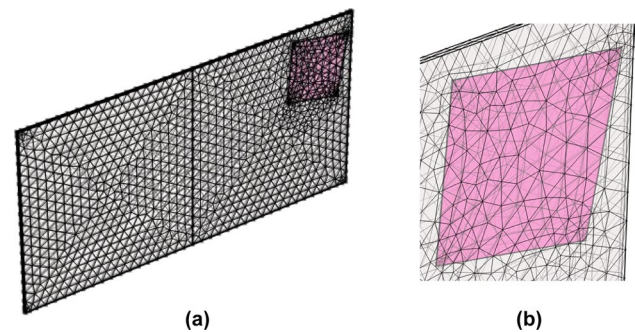
Fig. 7 Mesh used in numerical simulations: a overview and b details on the composite/inclusion interface
