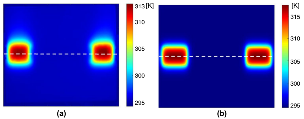
Fig. 17 Thermal image at the final instant of heating (120 s): a experiment and b numerical simulation
