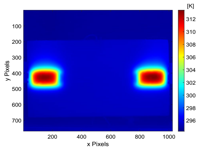
Fig. 9 Thermal image inherent to scenario 2 at the end of heating [K]
