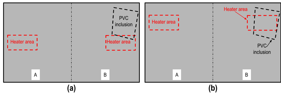
Fig. 16 Front view of numerical model: a scenario 2a and b scenario 2b
