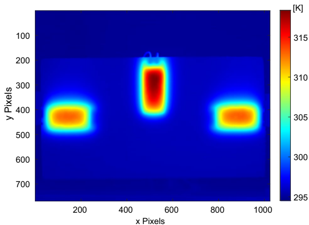
Fig. 13 Thermographic images for scenario 3 at the end of heating
