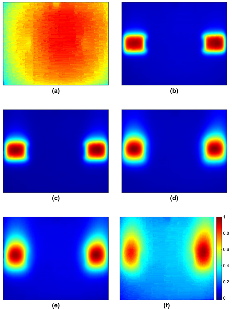
Fig. 10 Thermal images of excess temperature normalized for scenario 2: a 0 s, b 60 s, c 120 s, d 180, e 240 s, and f 420 s
