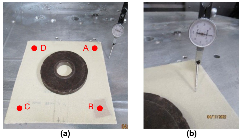
Fig. 3 Position of the composite plate on the measuring plane: a general view and b detail of the measuring probe on 0 to allow the piece zero procedure
