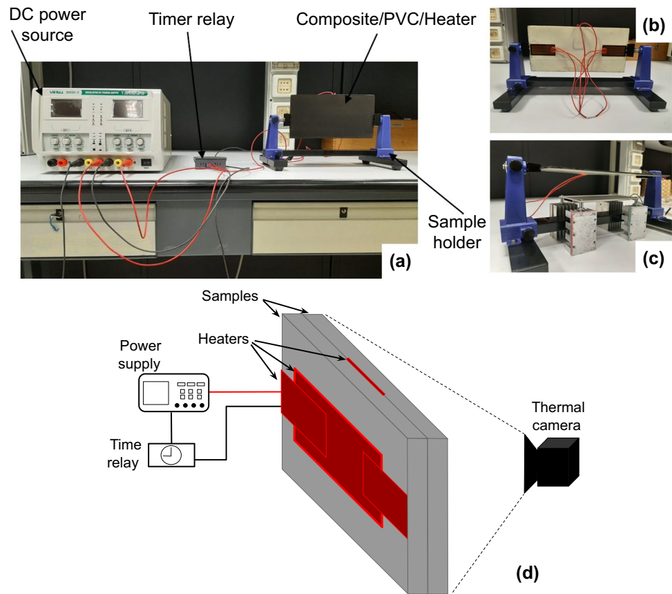
Fig. 1 Experimental setup with IR camera in the laboratory: a overview, b two heaters, c heater plate, and d schematic setup
