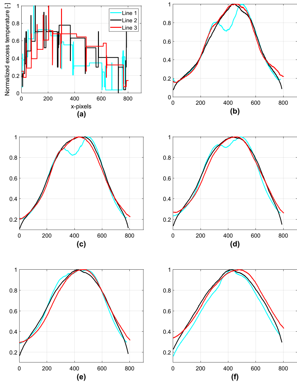
Fig. 15 Normalized excess temperature lines for scenario 4: a 0 s, b 60 s, c 120 s, d 180, e 240 s, and f 420 s
