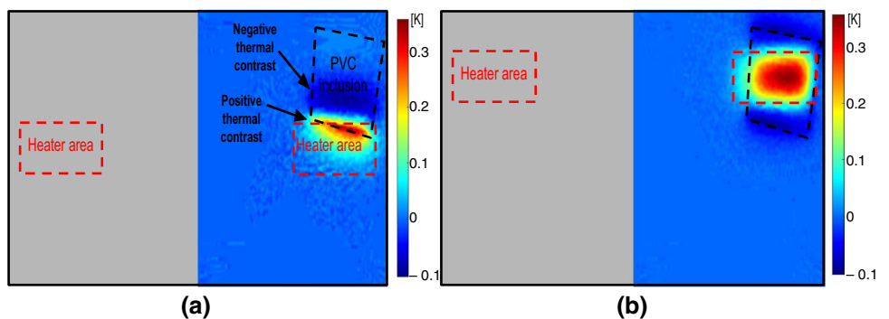
Fig. 19 Numerical thermal contrast at the end of heating ( t = 120 s): a scenario 2a and b scenario 2b
