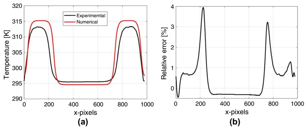
Fig. 18 Error between experimental and numerical temperatures: a absolute error and b relative error
