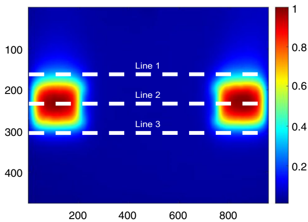
Fig. 11 Cut lines in the normalized thermographic image
