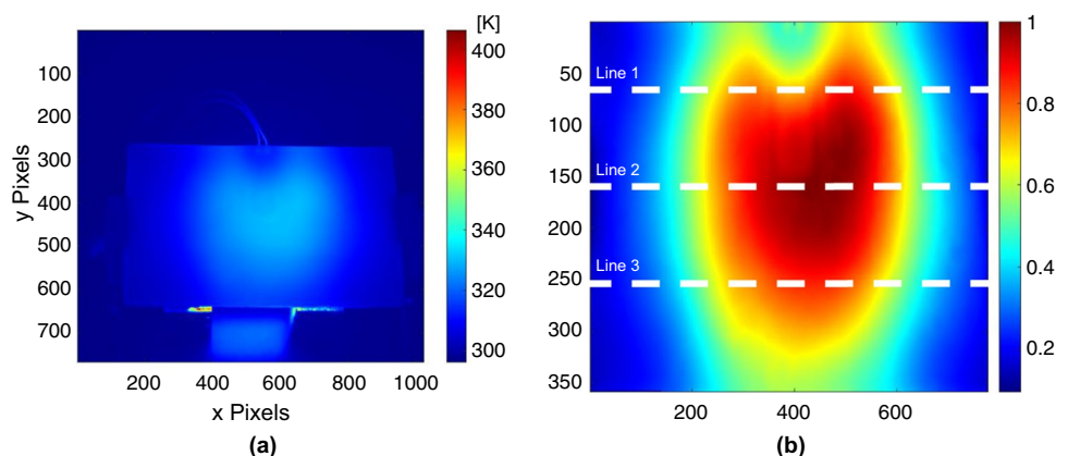
Fig. 14 Thermographic images for scenario 4 at the end of heating: a temperature distribution [K] and b normalized excess temperature distribution [-]
