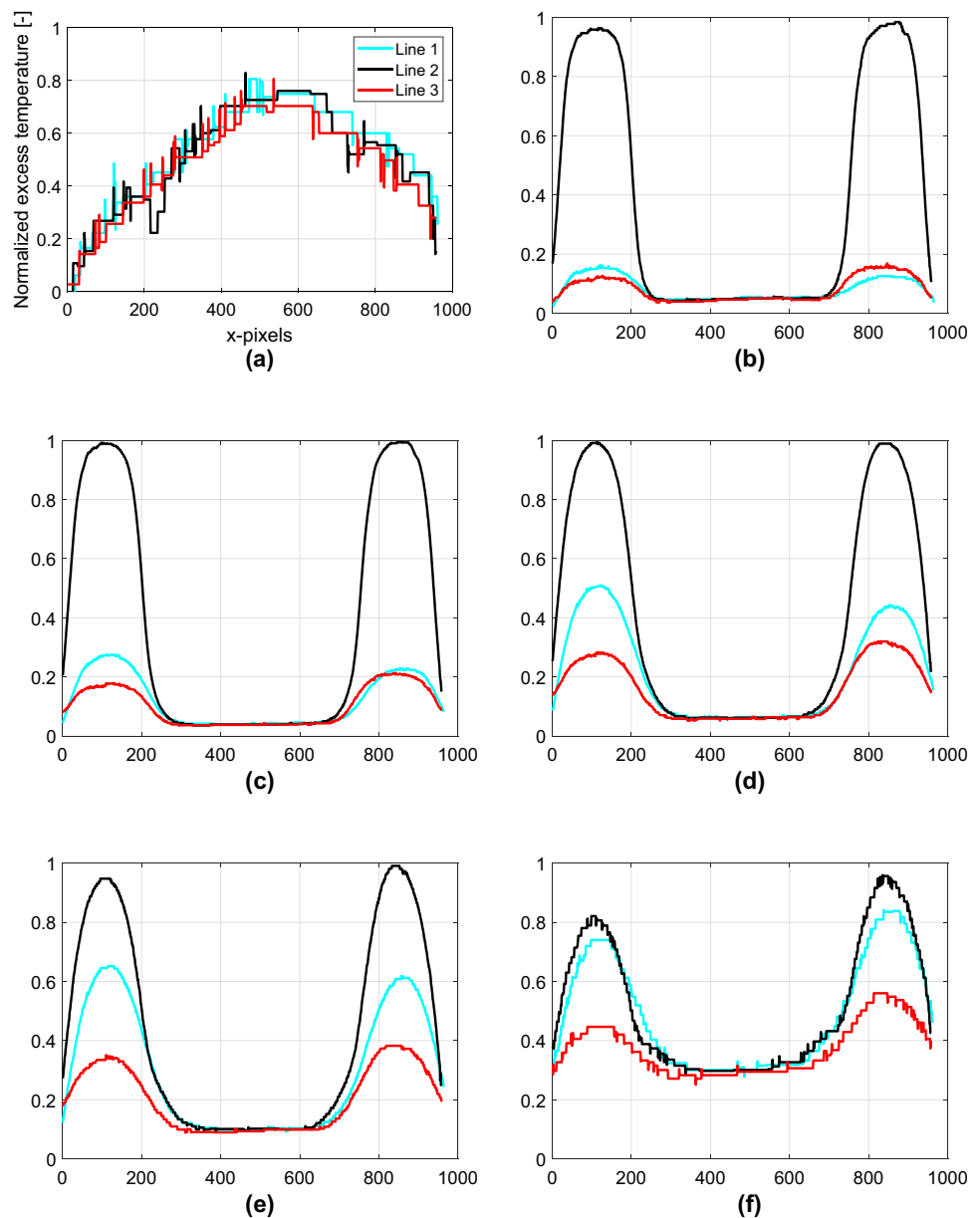
Fig. 11 Cut lines in the normalized thermographic image
