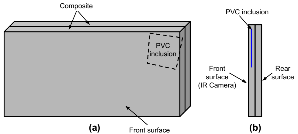
Fig. 5 Schematic drawing of composite material geometry and defect: a front surface and b side view
