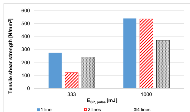
Fig. 25 Tensile shear strength versus E_{SP, \text{ pulse}} of PW lap joints of Al-SS
