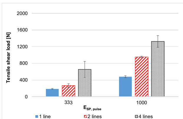
Fig. 21 Tensile shear load versus E_{SP, \text{ pulse}} of PW lap joints of Al-SS
