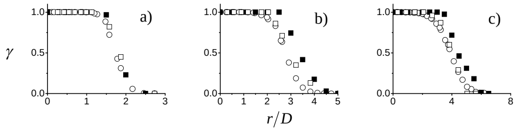
Fig. 12 Radial variation of scalar intermittency at (a) z/D=15 , (b) z/D=30 and (c) z/D=50 ( \circ Schefer and Dibble (2001), \blacksquare present LES, \square alternative LES).
