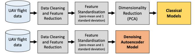
Fig. 12. Preprocessing pipelines various model types.
