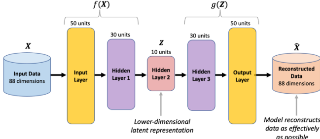
Fig. 10. Encoder-Decoder architecture representation.
