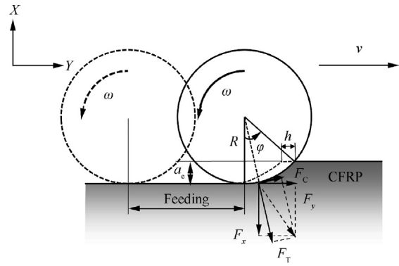
Fig. 7 Schematic of up-milling configuration.
