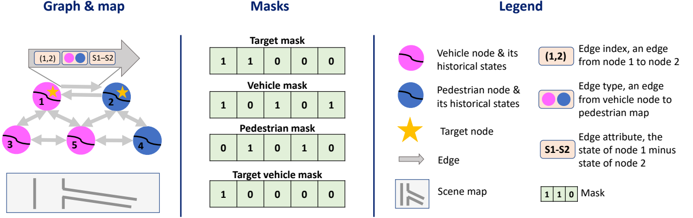
Fig. 4. Processed data. Left , the directed edge-featured heterogeneous interaction graph (top) obtained after processing and the map (bottom). Middle , the mask vectors. Right , the legend of this figure. The interaction graph is constructed via close connection strategy, where each node is only connected to its neighboring nodes via directed edges. A directed edge is identified via its edge index and contains edge type and edge attribute.
