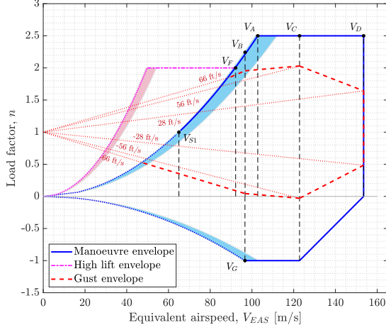
Fig. 7 Design operational envelope.
