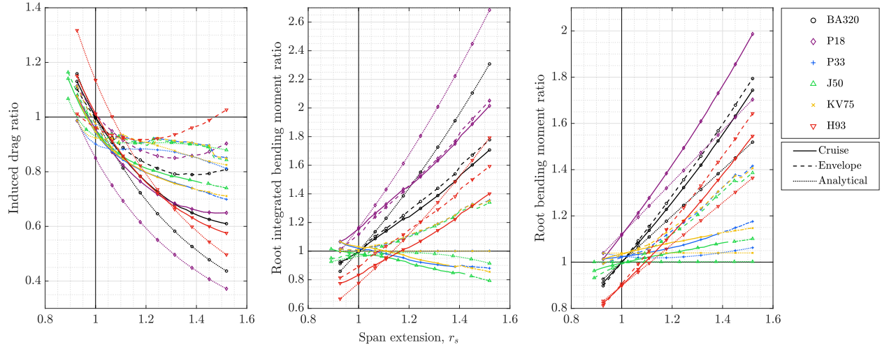
Fig. 11 Aero-structural trends due to aerodynamic loads for span extension against the baseline configuration.
