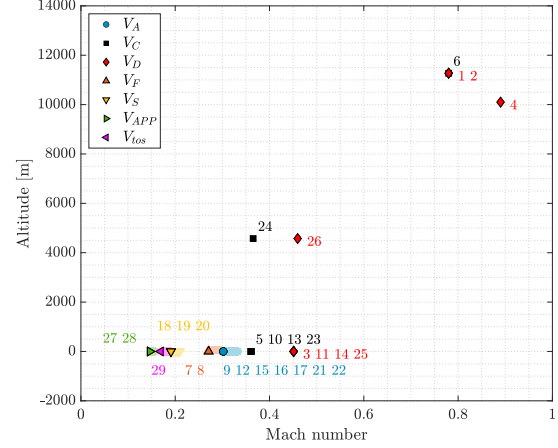
Fig. 8 Flight points assessed and manoeuvre ID.
