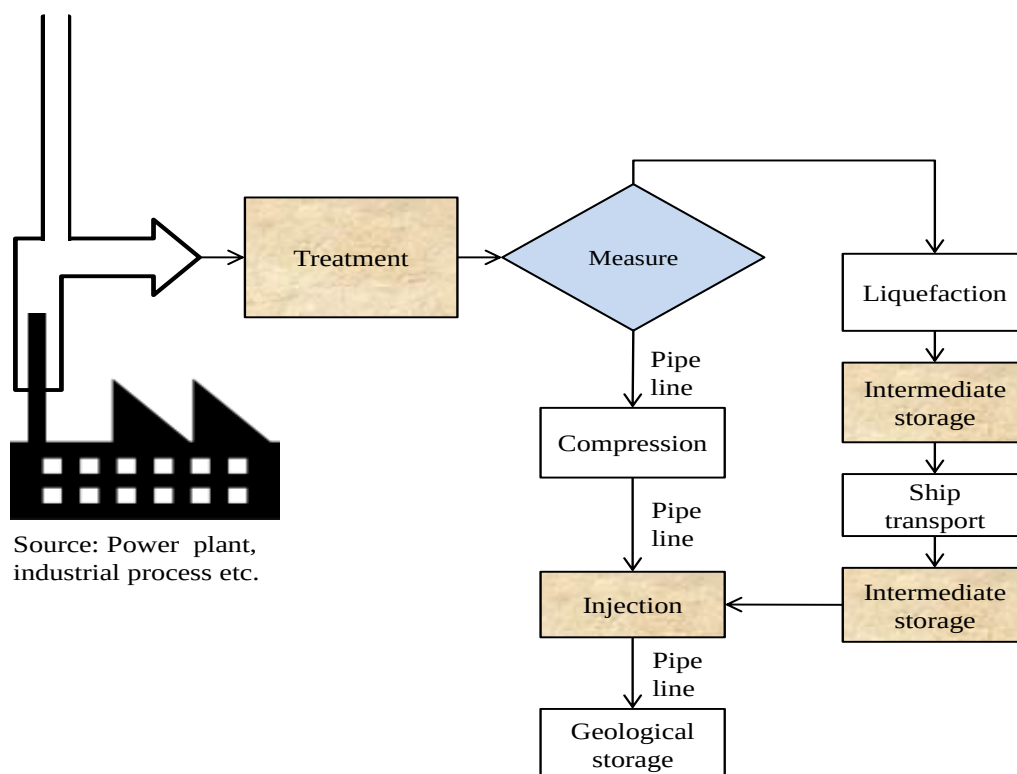
Figure 1: Liquefaction and compression transport schemes (Adapted from Spinelli et al. [32]. Copyright 2012 The International Society of Offshore and Polar Engineers)
