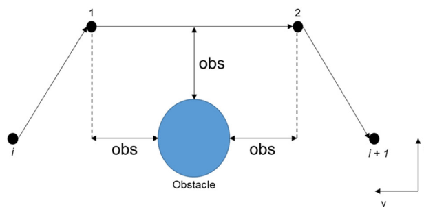
Fig. 1 The avoidance motion taken by the robot to avoid a collision with an obstacle where i represents the current position, i + 1 represents the next waypoint, 1 and 2 represent avoidance waypoints, obs represents the proximity setting, and the obstacle is either the head, left hand or right hand (depending on which is closest to TCP, and then in priority order of avoiding the head over the hands)
