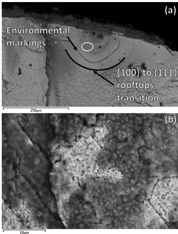
Fig. 9. BSE, SEM images of an 800 MPa, 5 \mu\text{g}/\text{cm}^2/\text{h} , 1-1-1-1 specimen (a) Fracture face showing transition between \{100\} and \{111\} [13] (b) Higher magnification of circled location in image (a) showing corrosion product build up on fracture surface.
