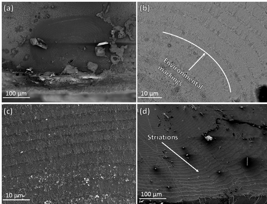
Fig. 8. Fracture face images of specimen exposed to 750 MPa, 1-1-1-1, 5 \mu\text{g}/\text{cm}^2/\text{h} deposit flux (a) Secondary electron (SE) image of \{100\} crack initiation and propagation showing environmental oxidation/corrosion banding close to initiation point (b) Back scattered electron (BSE) image of environmental oxidation/corrosion banding (c) SE image of environmental oxidation/corrosion banding (d) SE image of \{111\} fatigue striations prior to mechanical overload located on \{111\} facets.
