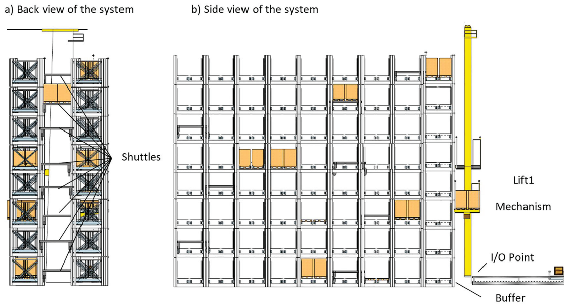
Figure 1. A c -SBSRS design. (a) Back view of the system. (b) Side view of the system.
