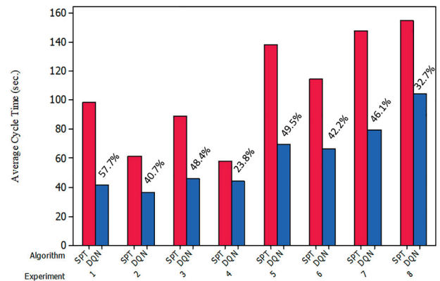
Figure 9. Comparison of SPT and DQN selection policies for C_{avg} .
