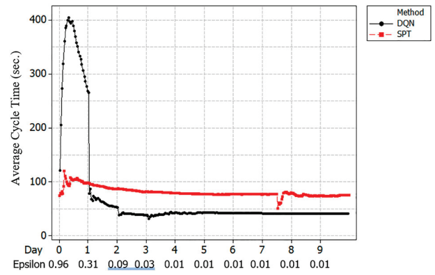
Figure 8. Average cycle time of each day.
