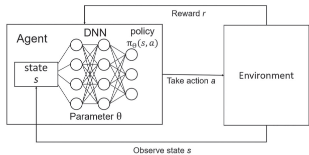
Figure 3. Agent behaviour in DQN (adopted from Mao et al. 2016).
