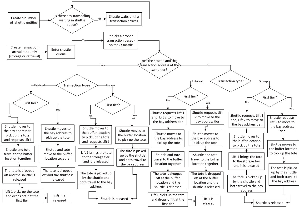
Figure 6. Flow chart of the agent-based simulation model.
