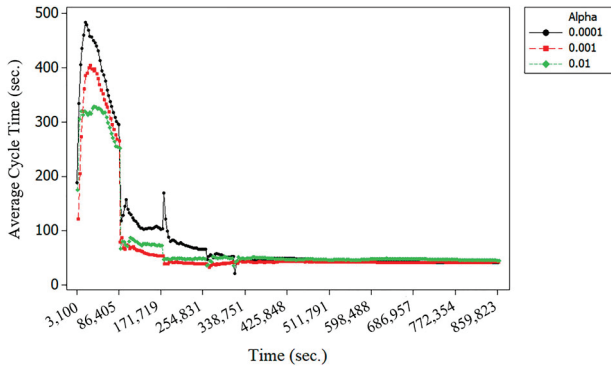
Figure 7. DQN results under three different learning rate scenarios.
