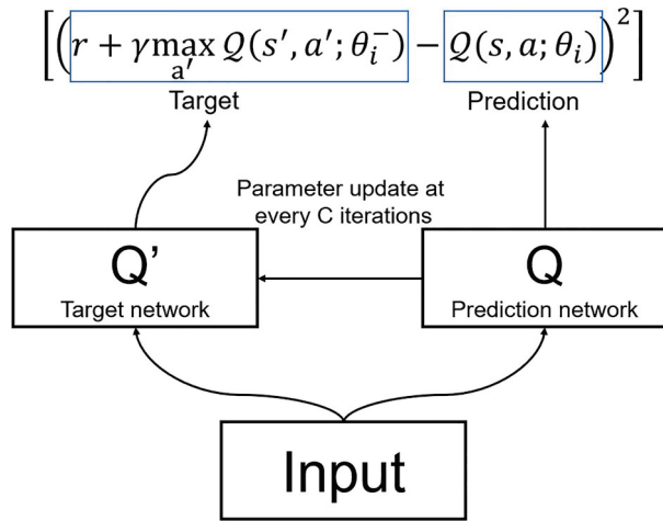
Figure 4. Updating target network by using prediction network (adopted from Choudhary 2019).
