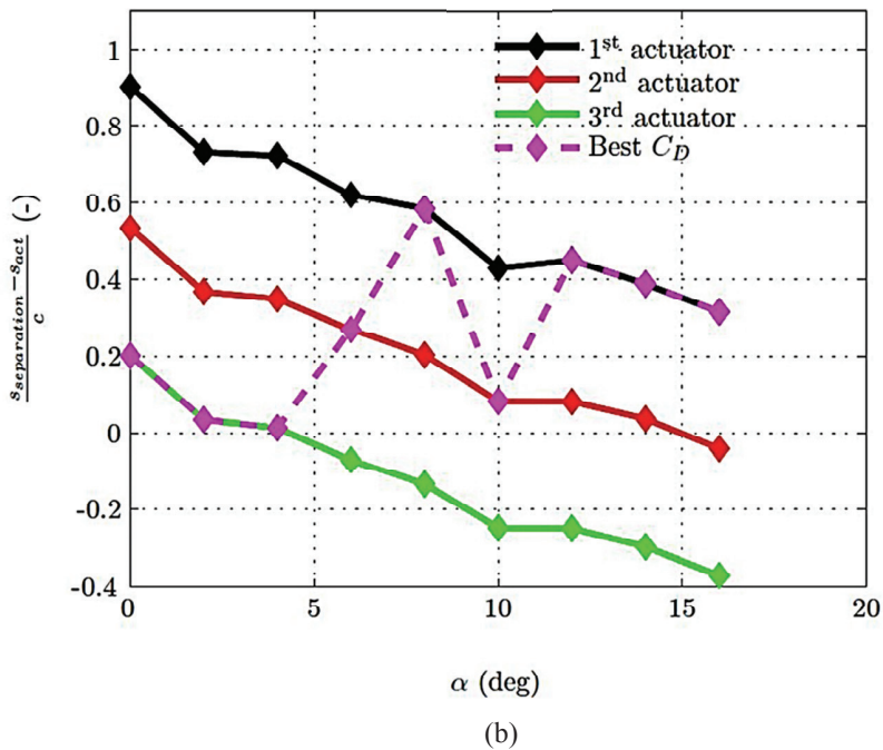
Fig. 4 Evolution of the non-dimensional curvilinear distances between the flow separation points and the actuator locations with the angle of attack for Re = 35000 : (a): actuators associated with the best C_L connected with a dotted blue line; (b): actuators associated with the best C_D joined with a dotted magenta line.
